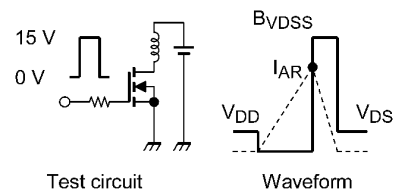
Fig. 9.15 Test Circuit/Waveform
