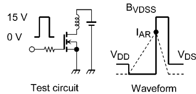
Fig. 8.15 Test Circuit/Waveform
