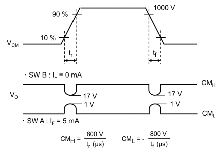
Fig. 12.1.8 Common-Mode Transient Immunity Test Circuit and Waveform
