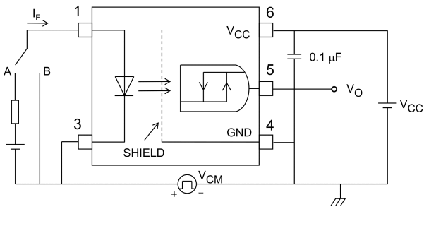
Fig. 12.1.9 Common-Mode Transient Immunity Test Circuit and Waveform
