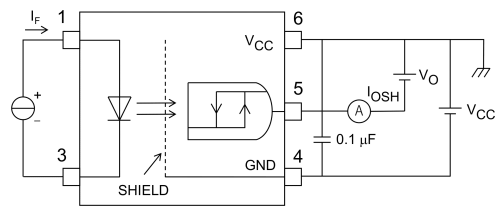
Fig. 12.1.6 I_{OSH} Test Circuit
