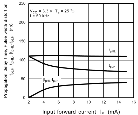
Fig. 12.2.24 t_{pHL}, t_{pLH}, |t_{pHL} - t_{pLH}| - I_F (Test Circuit Fig. 12.1.8)
