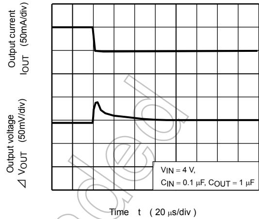
TCR5SB30U ( I_{OUT} = 100\text{m to }50\text{mA} )
