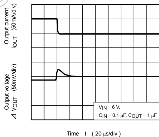
TCR5SB50U ( I_{OUT} = 100\text{m to }50\text{mA} )
