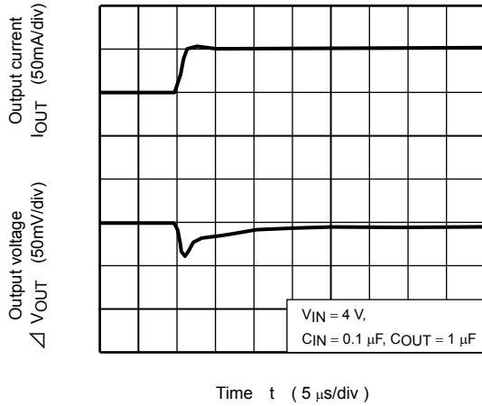
TCR5SB30U ( I_{OUT} = 50\text{m to }100\text{mA} )
