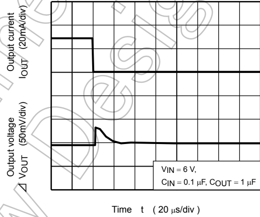
TCR5SB50U ( I_{OUT} = 30\text{m to }1\text{mA} )
