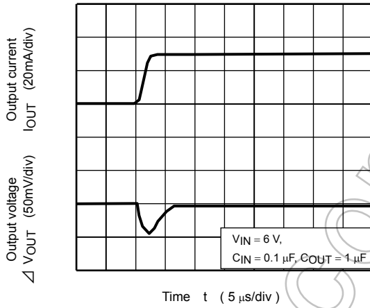
TCR5SB50U ( I_{OUT} = 1\text{m to }30\text{mA} )
