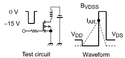
Fig. 9.15 Test Circuit/Waveform
