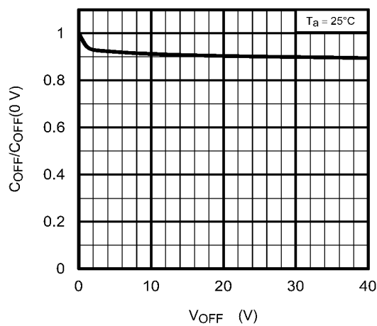
Fig. 12.1.11 C_{OFF}/C_{OFF(0V)} - V_{OFF}
