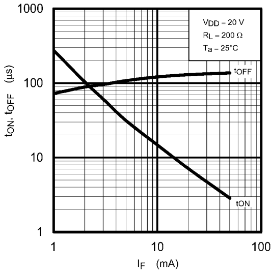
Fig. 12.1.7 t_{ON}, t_{OFF} - I_F
