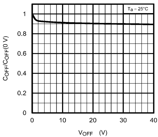
図 12.1.11 C_{OFF}/C_{OFF(0V)} - V_{OFF}
