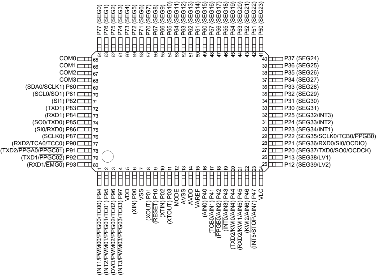
TMP89FW24ADFG (QFP80-P-1420-0.80M)
