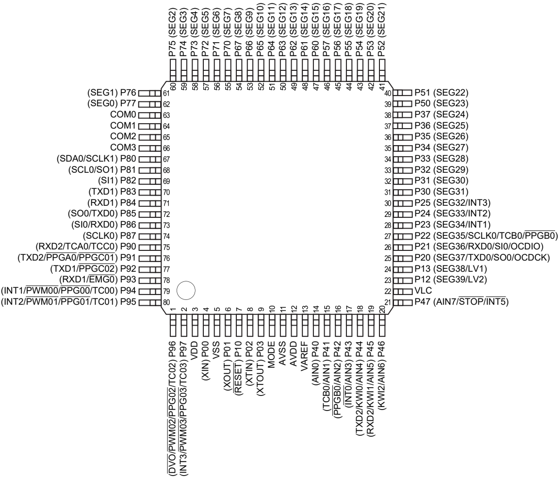
TMP89FW24AFG (LQFP80-P-1212-0.50F)
