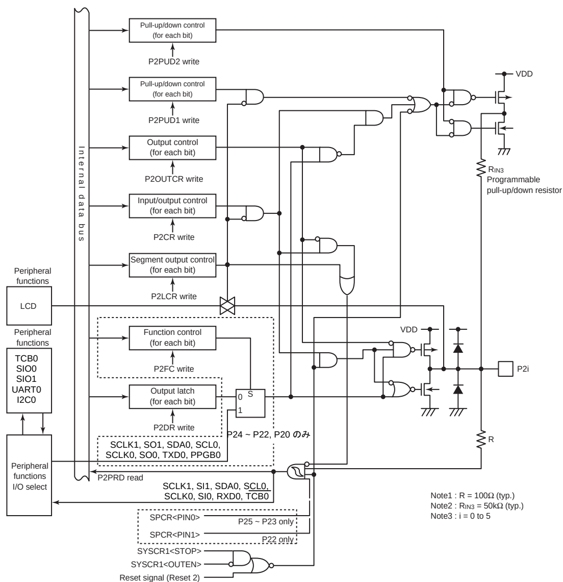
Figure 8-5 Port P2
