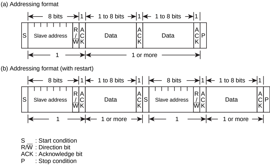
Figure 20-2 Data Format of I 2 C Bus
