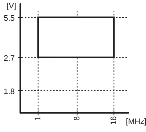
High-frequency clock(fc) frequency range
