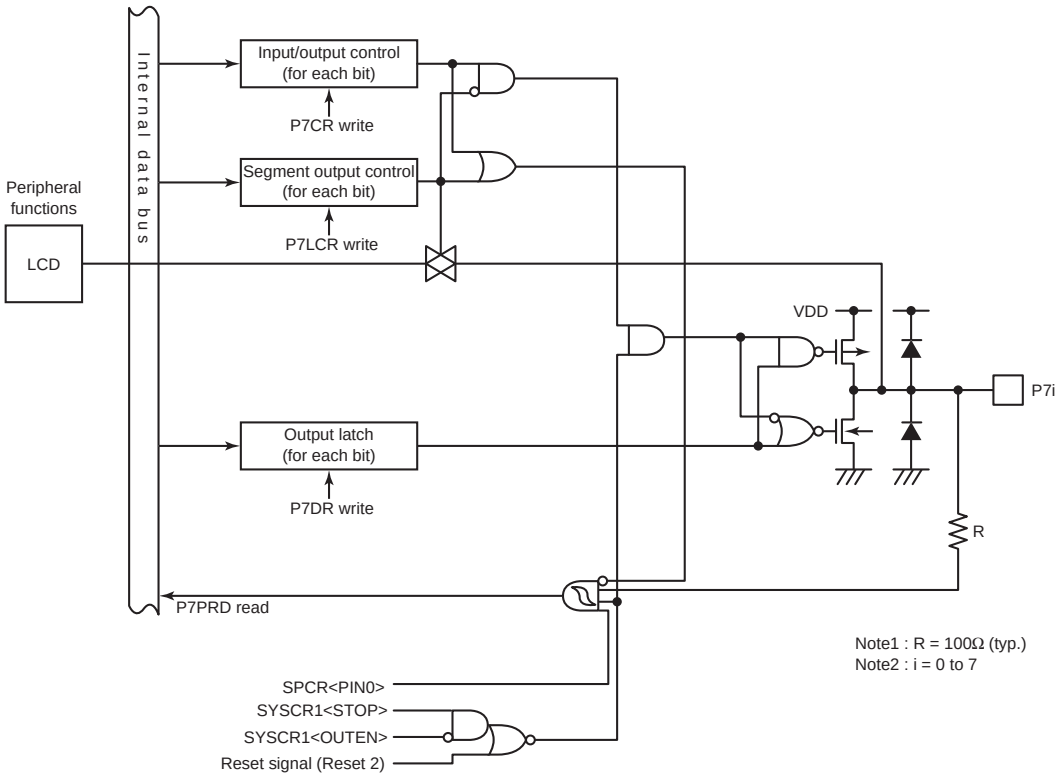
Figure 8-9 Port P7
