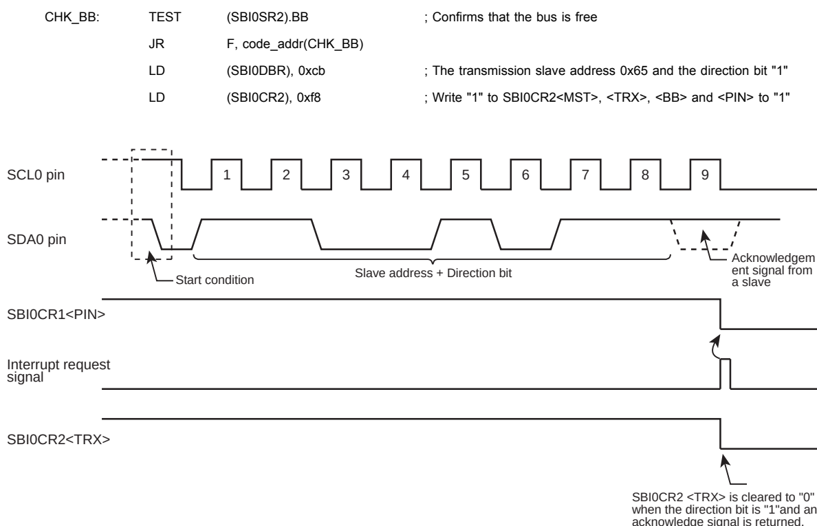
Figure 20-17 Generating the Start Condition and the Slave Address
