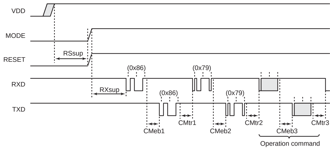
Figure 26-6 Reset Timing
