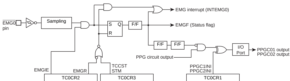
Figure 15-22 \overline{\text{EMG0}} Pin
