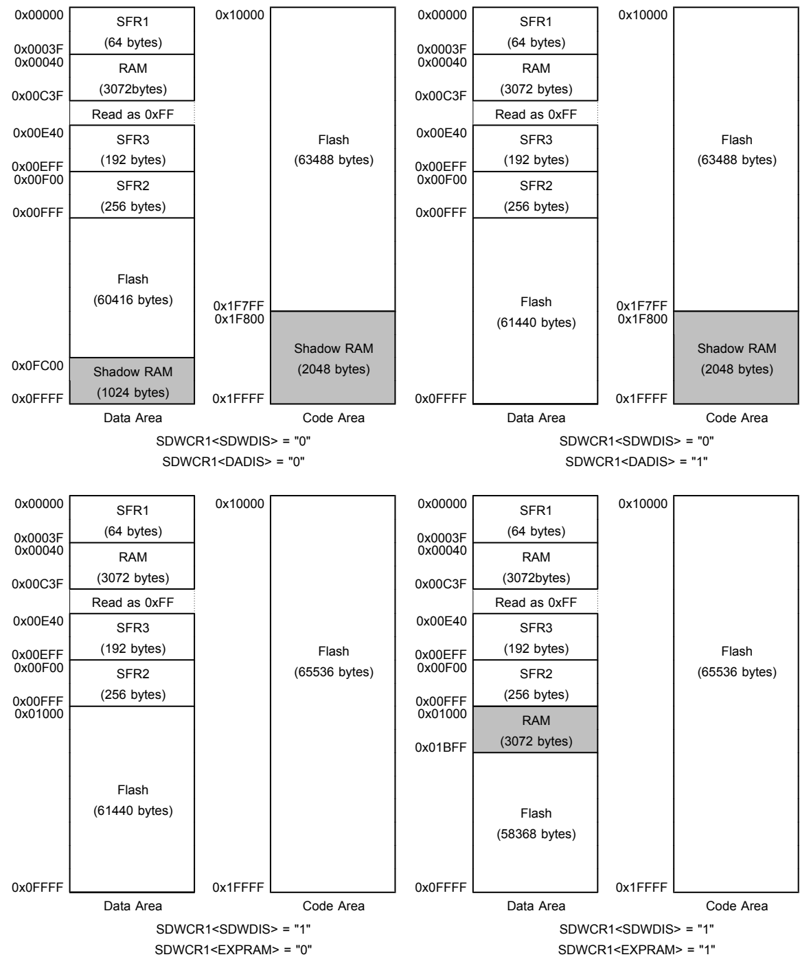
Figure 25-2 Memory Map
