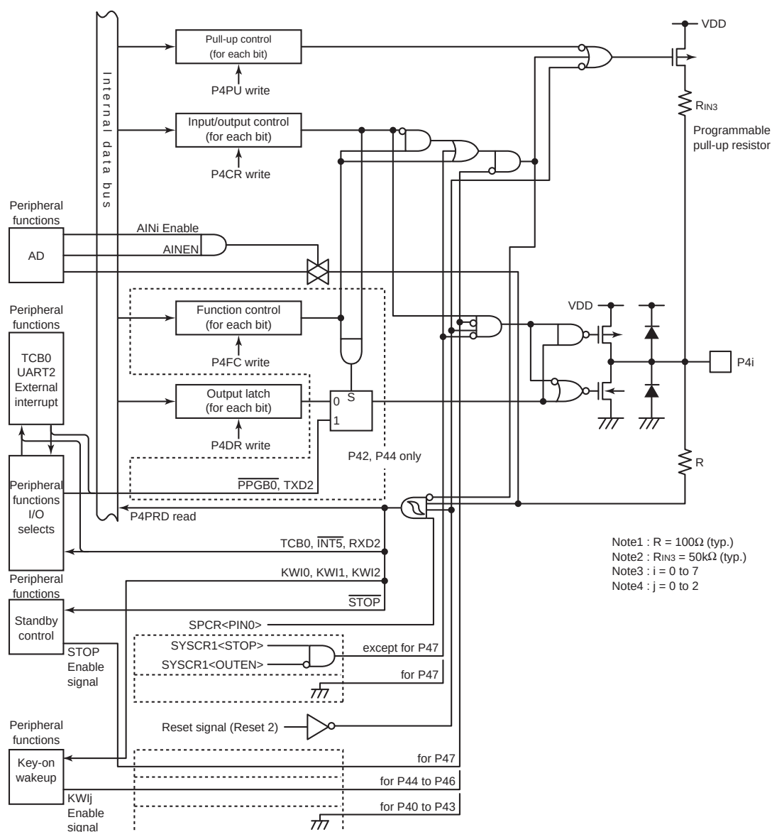
Figure 8-6 Port P4
