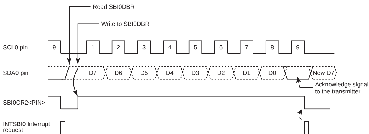
Figure 20-19 Example when SBI0CR1&lt;BC&gt;="000" and SBI0CR1&lt;ACK&gt;="1"
