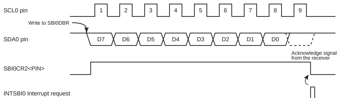
Figure 20-18 Example when SBI0CR1&lt;BC&gt;="000" and SBI0CR1&lt;ACK&gt;="1"
