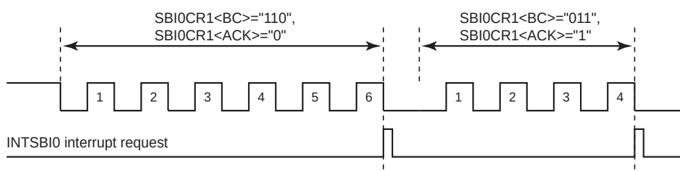
Figure 20-5 Number of Clocks for Data Transfer and SBI0CR1<BC> and SBI0CR1<ACK>
