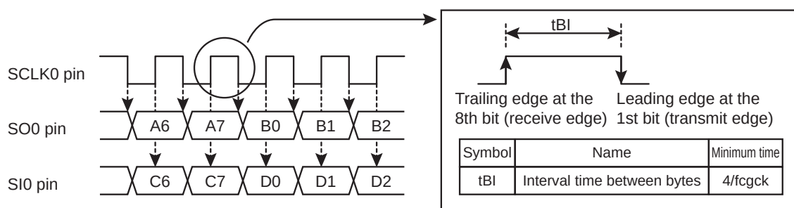
Figure 19-18 Interval time between bytes
