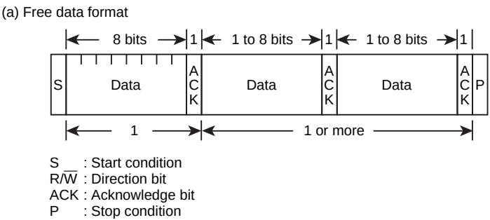
Figure 20-3 Free Data Format
