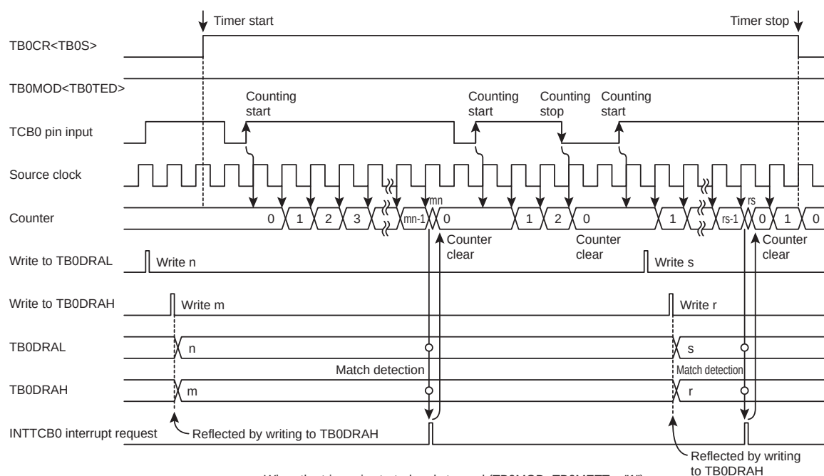
Figure 14-4 External Trigger Timer Timing Chart
