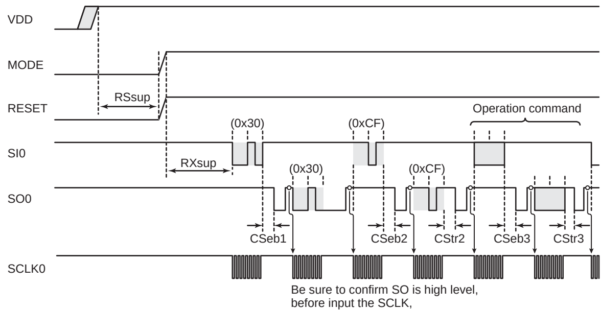
Figure 26-17 Reset Timing
