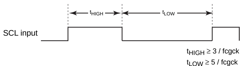
Figure 20-7 SCL Input
