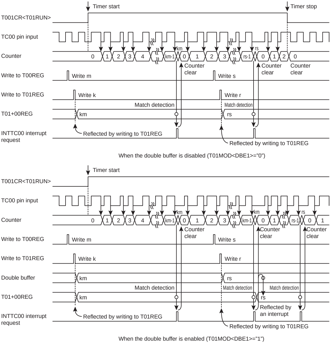
Figure 16-12 16-bit Event Counter Mode Timing Chart
