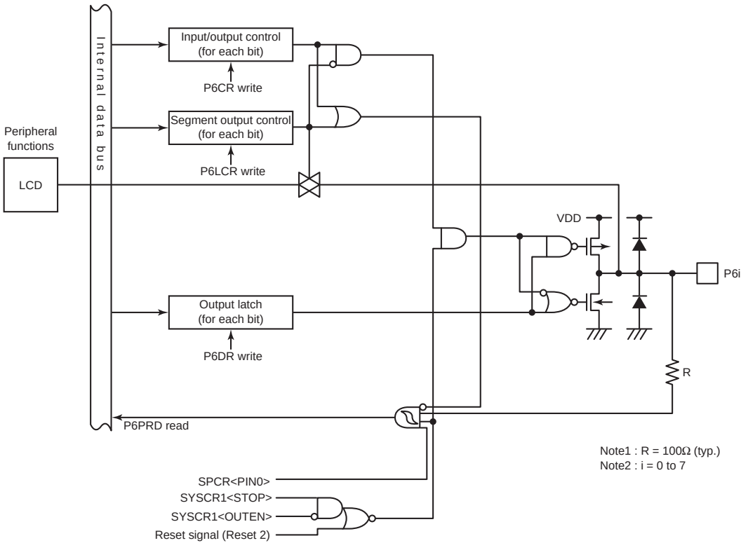
Figure 8-8 Port P6
