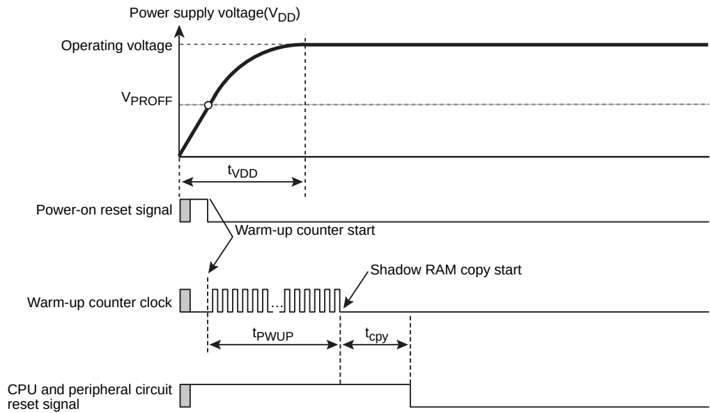
Figure 29-4 Power-on Reset Operation Timing
