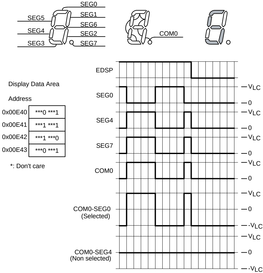
Figure 23-12 Static Drive
