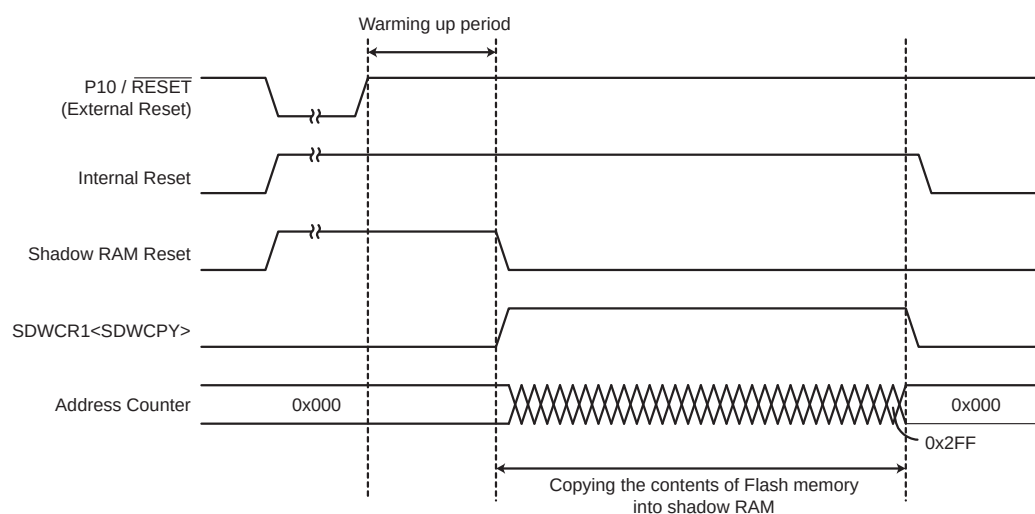
Figure 25-3 Copy Operation Timing at Reset
