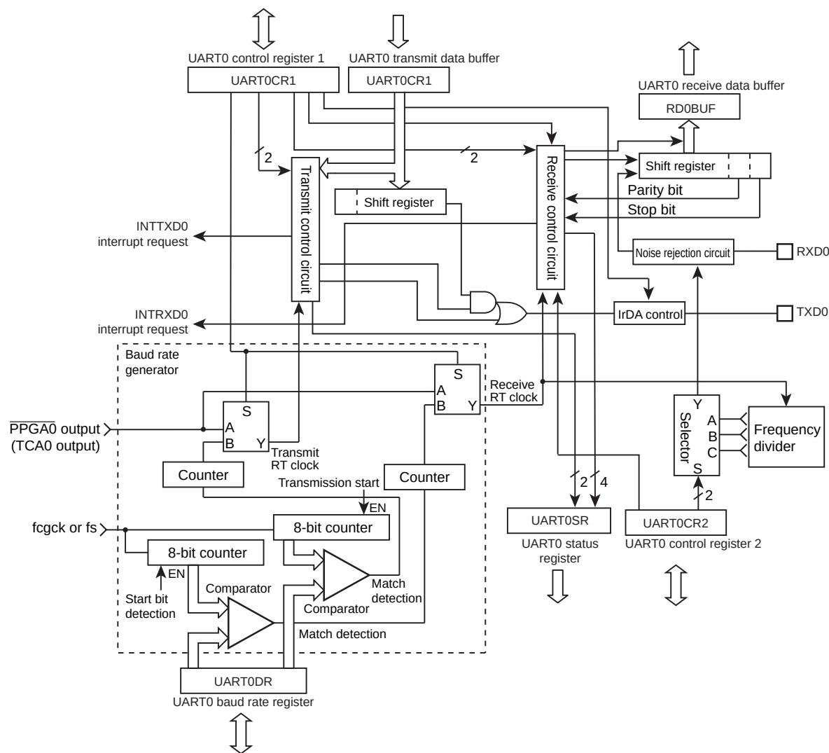
Figure 18-1 Asynchronous Serial Interface (UART)
