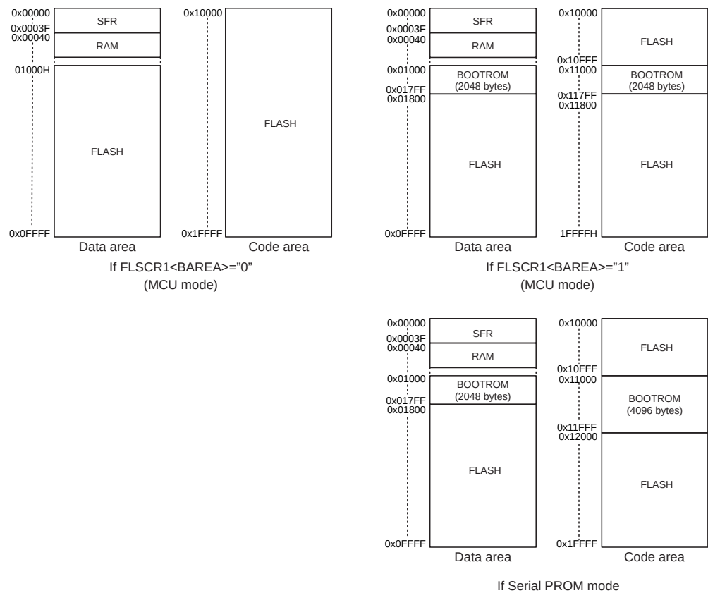
Figure 26-3 Memory Mapping
