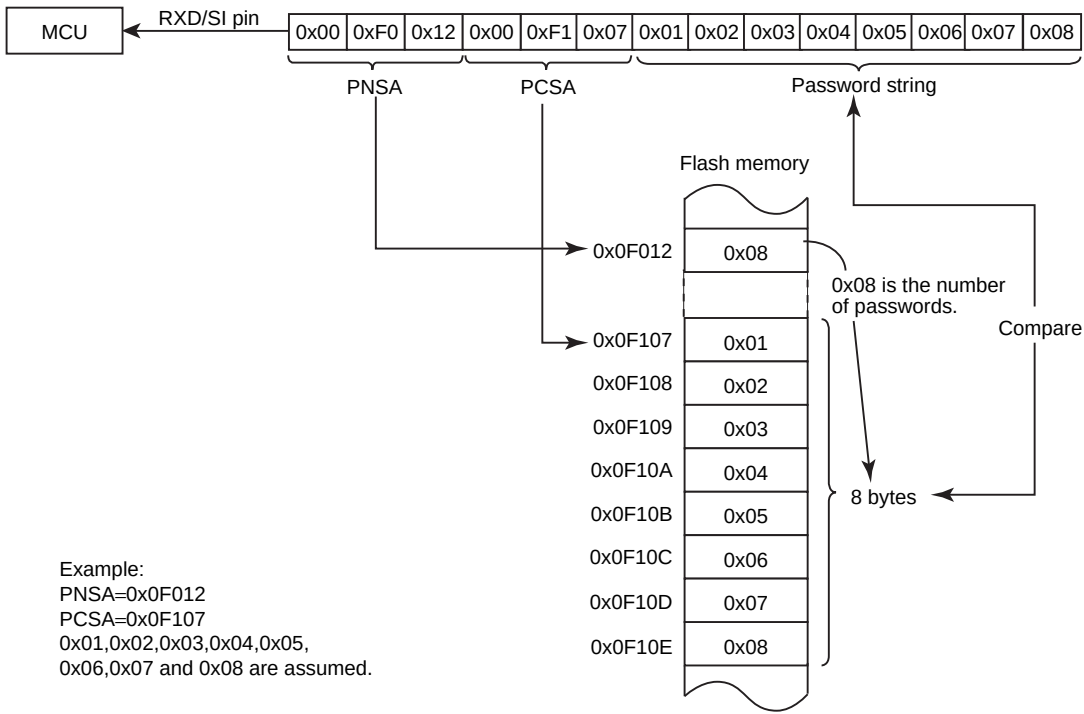
Figure 26-4 Example of How a Password Is Transmitted
