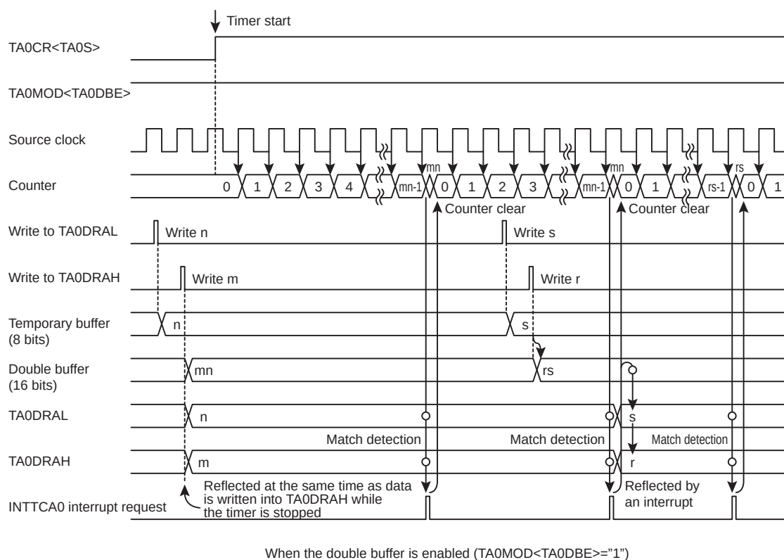
Figure 13-2 Timer Mode Timing Chart
