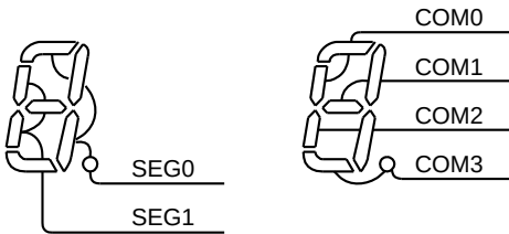
Figure 23-6 Example of COM and SEG Pin Connections (1/4 Duty)
