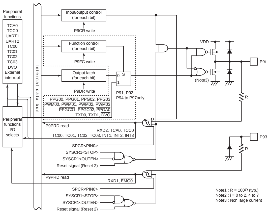
Figure 8-10 Port P9
