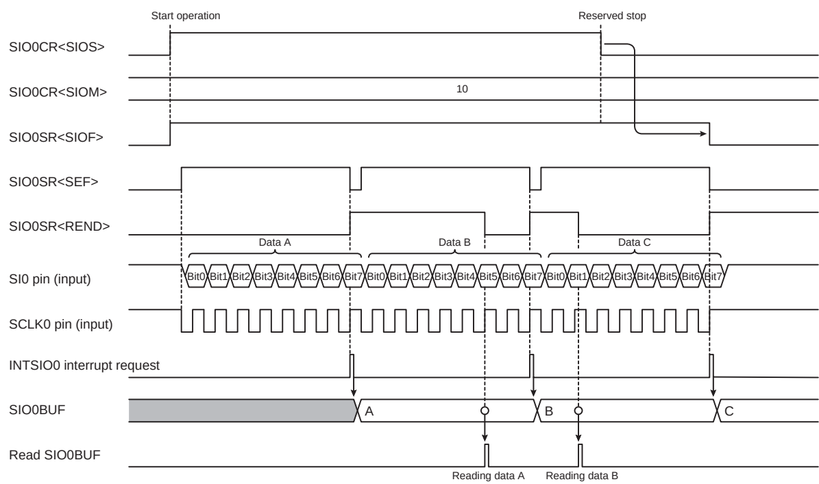
Figure 19-11 8-bit Receive Mode (External Clock and Reserved Stop)
