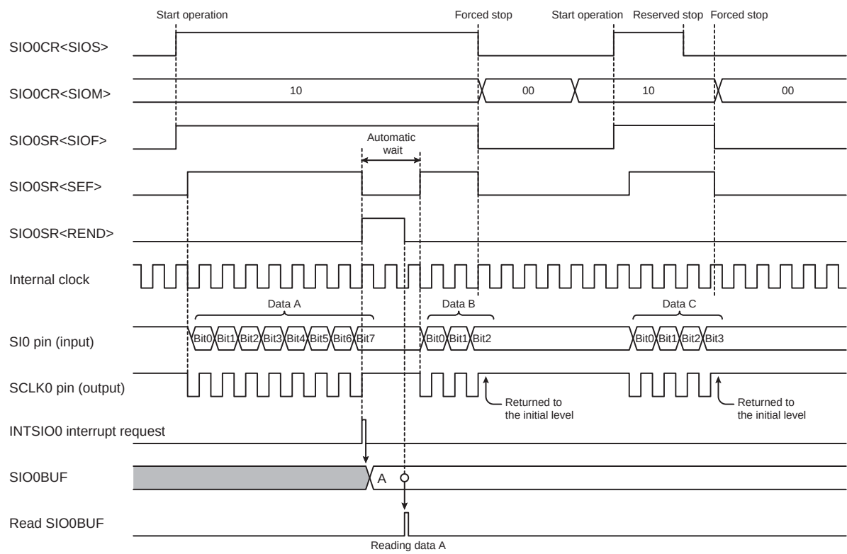
Figure 19-10 8-bit Receive Mode (Internal Clock and Forced Stop)
