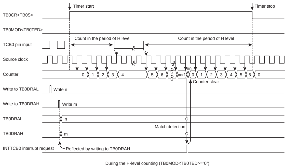
Figure 14-6 Window Mode Timing Chart
