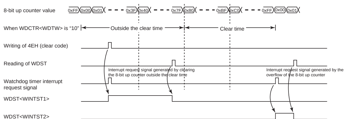
Figure 5-4 Changes in the Watchdog Timer Status
