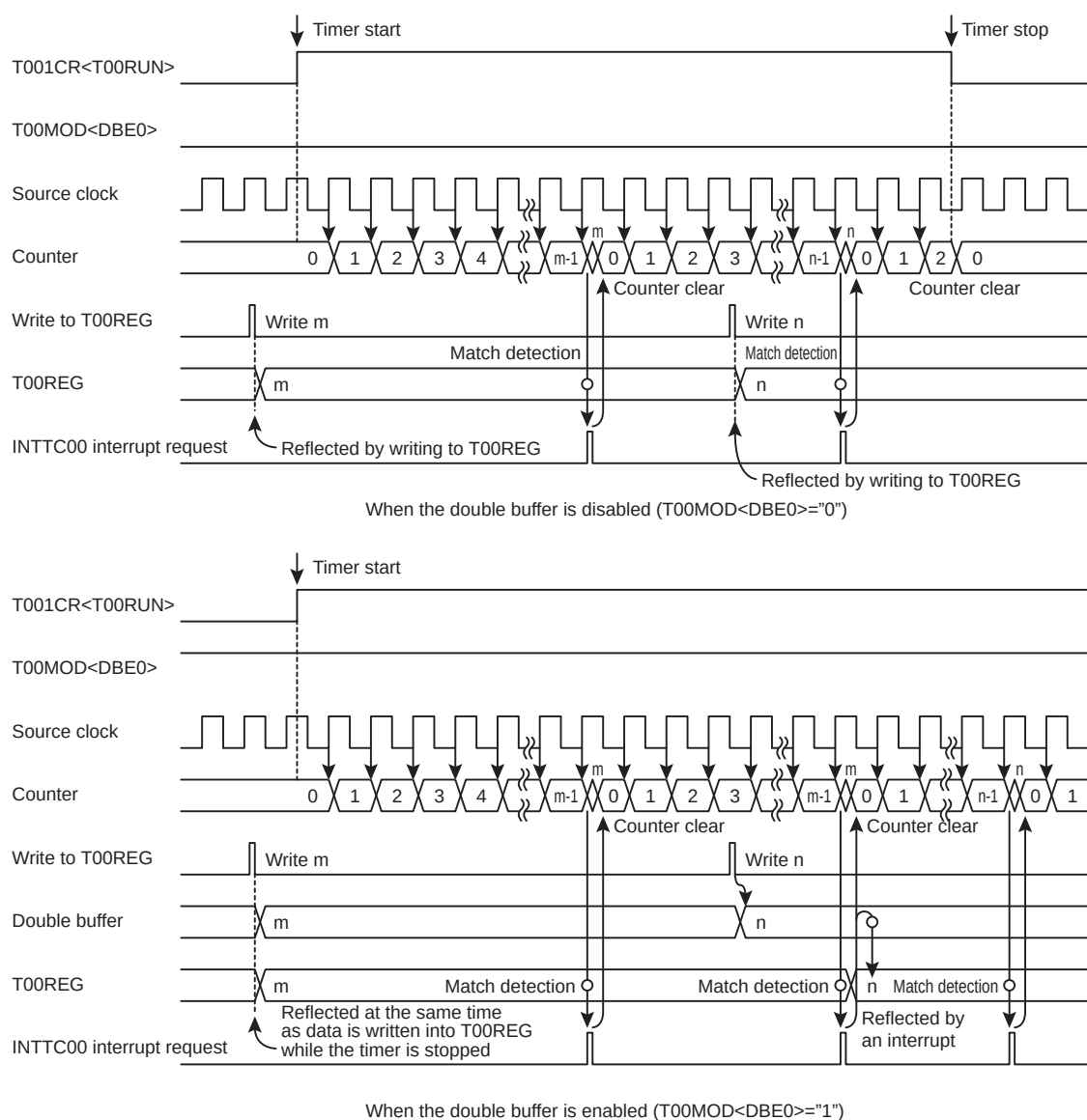
Figure 16-2 Timer Mode Timing Chart
