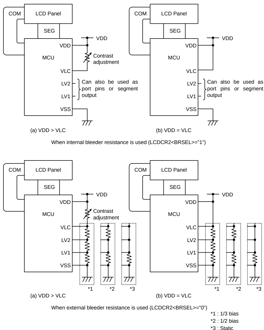
Figure 23-4 Connection Examples
