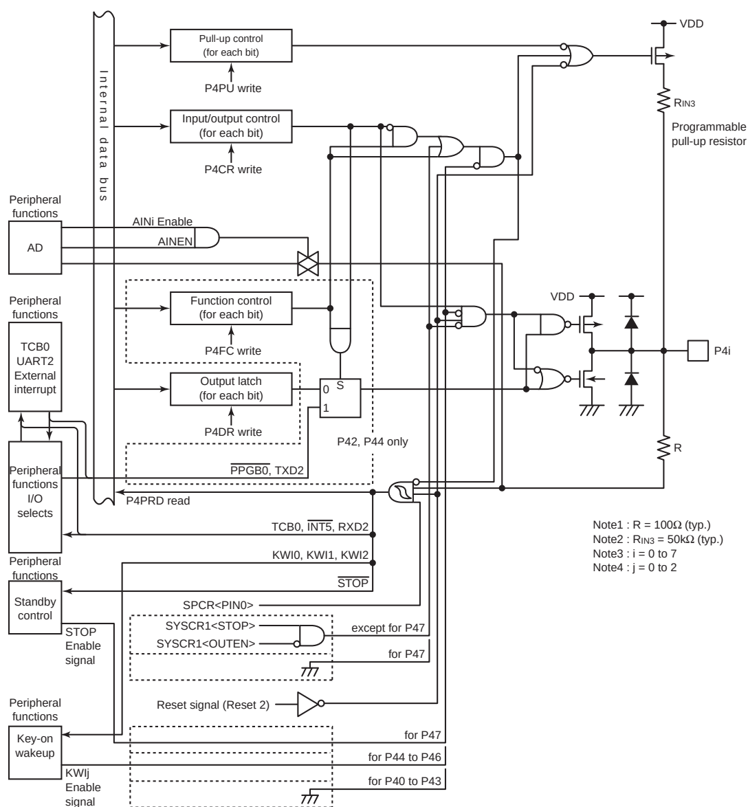
Figure 8-7 Port P4
