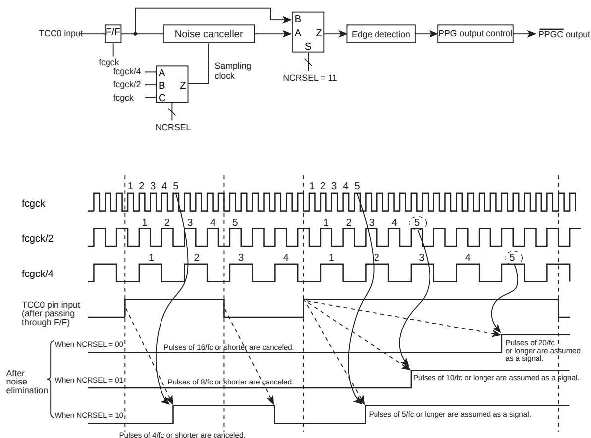
Figure 15-19 Noise Canceller Operation
