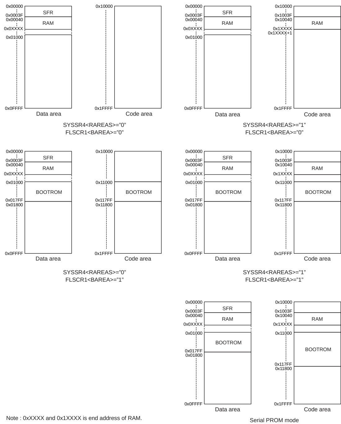
Figure 24-2 Show/Hide Switching for BOOTROM and RAM
