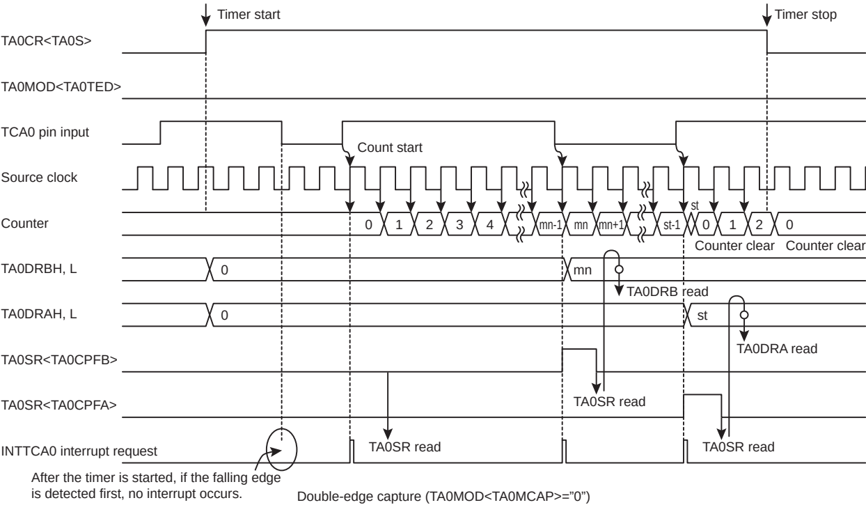
Figure 13-7 Pulse Width Measurement Mode Timing Chart
