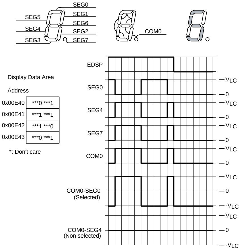
Figure 23-12 Static Drive
