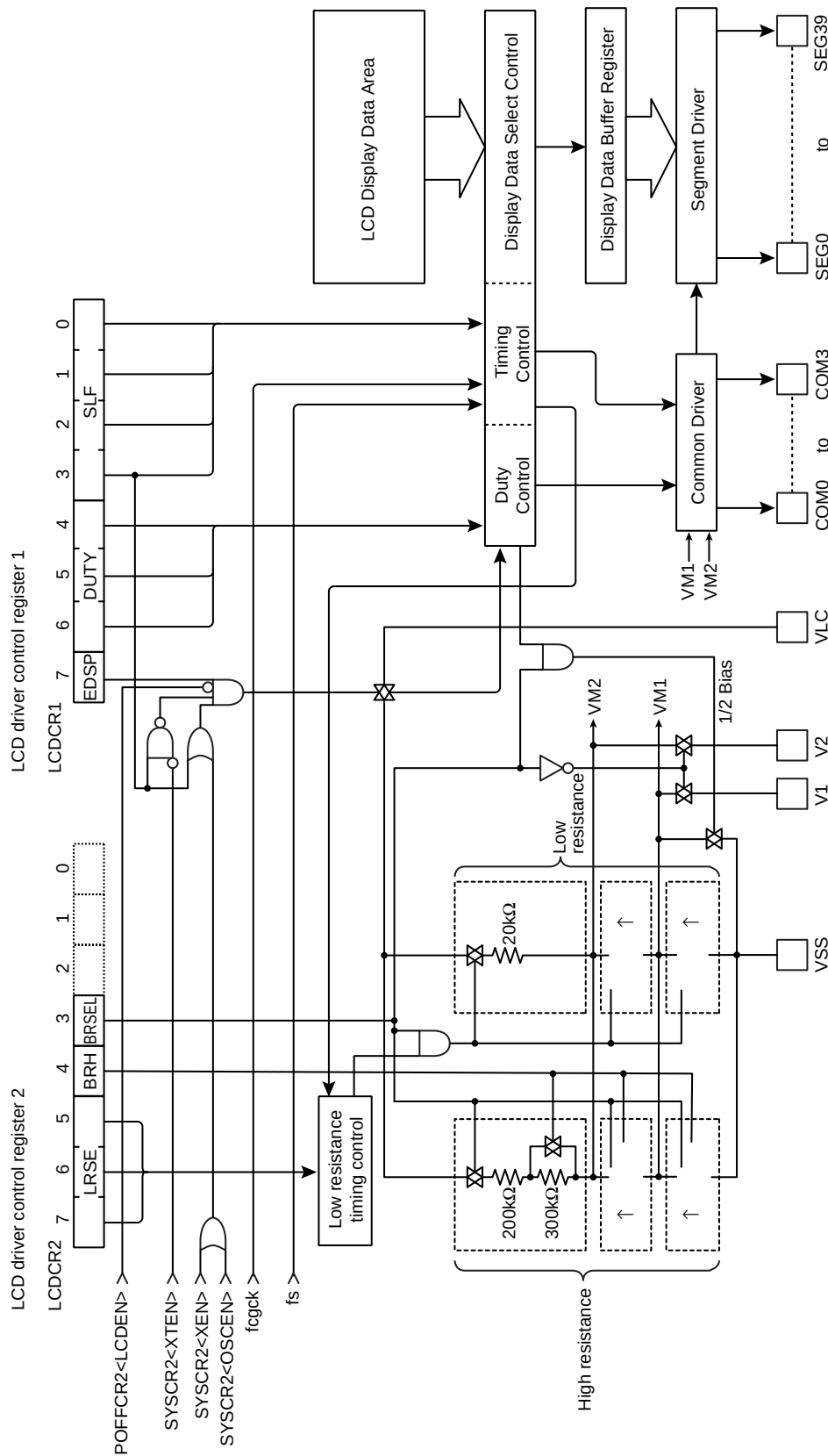
Figure 23-1 LCD Driver
