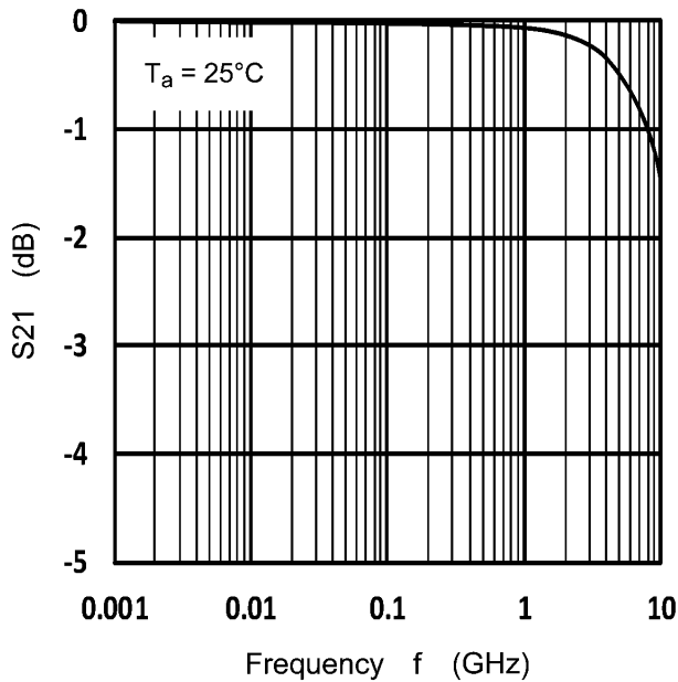
図 10.1 S_{21} - f
