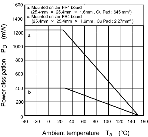
Fig. 8.14 P_D - T_a
