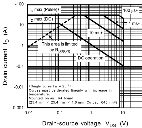
Fig. 8.15 Safe Operating Area
