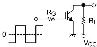
Fig. 6.2.1 Test Circuit of Switching Time
