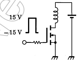
TEST CIRCUIT
