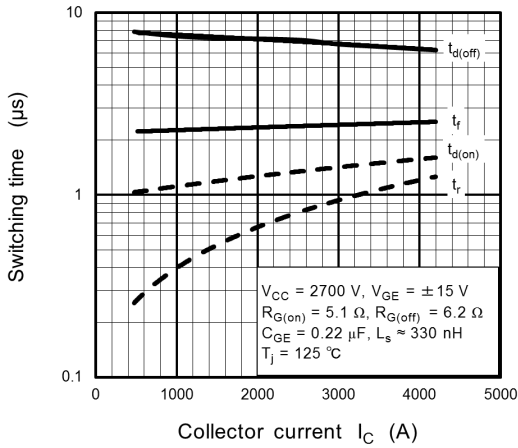
Fig. 7.7 t_{d(off)}, t_r, t_{d(on)}, t_r - I_C
