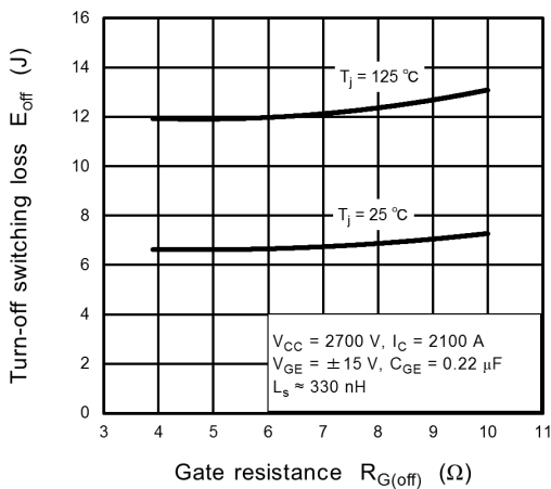
Fig. 7.9 E_{off} - R_{G(off)}
