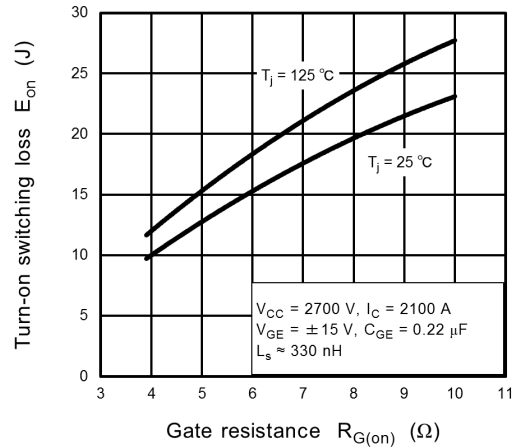
Fig. 7.8 E_{on} - R_{G(on)}
