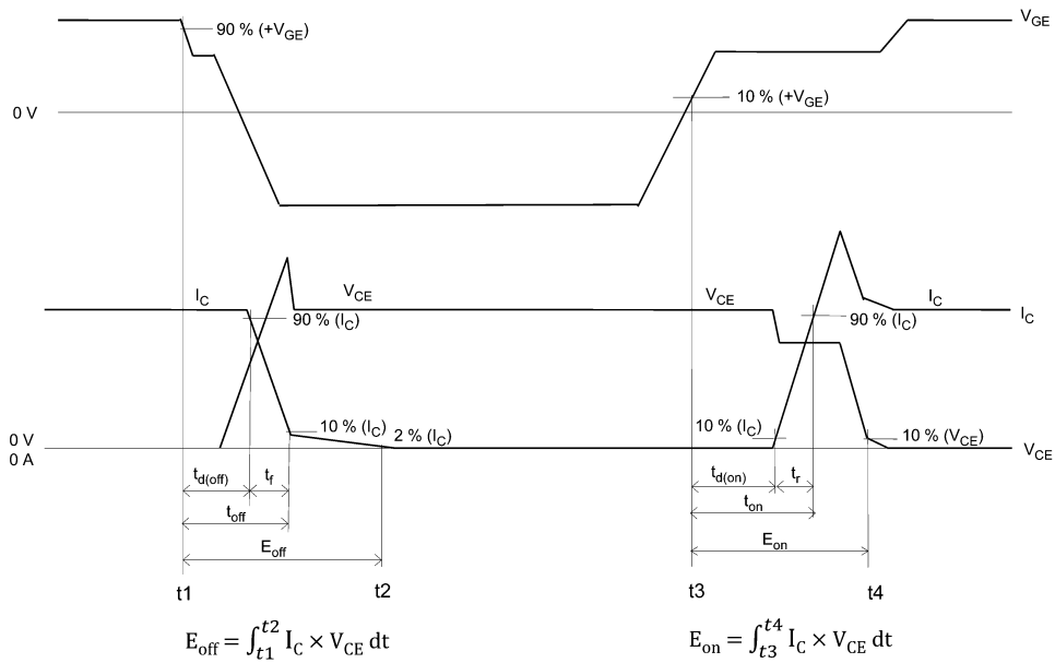
Fig. 6.2 Timing Chart
