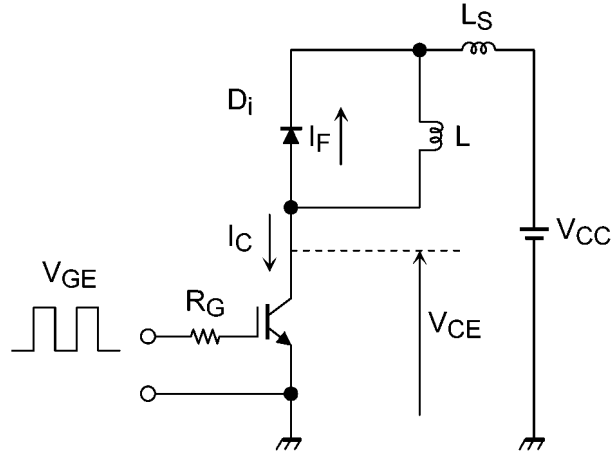
Fig. 6.1 Test Circuit
