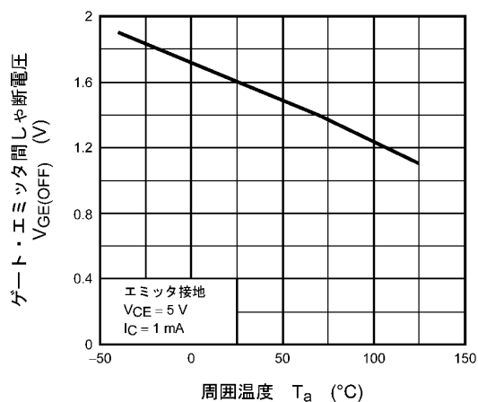
図 9.7 V_{GE(OFF)} - T_a
