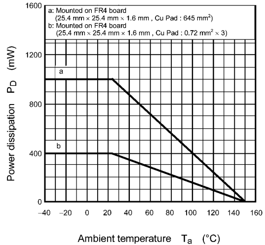
Fig. 8.14 P_D - T_a
