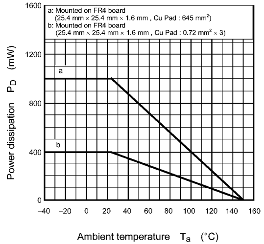
Fig. 8.14 P_D - T_a
