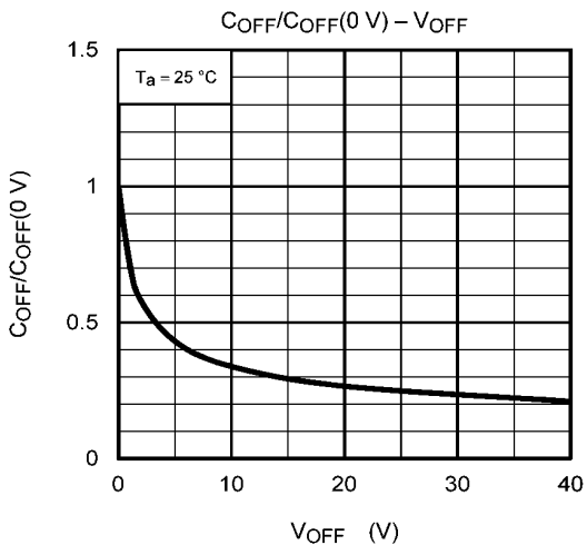
図 12.1.11 C_{OFF}/C_{OFF}(0V) - V_{OFF}
