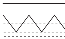
AMPSEL=1/2VDD, OFFSET=2/8VDD
