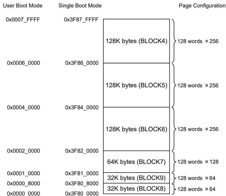
Figure 31-10 Block Configuration of Flash Memory (TMPM369DFDG/XBG)
