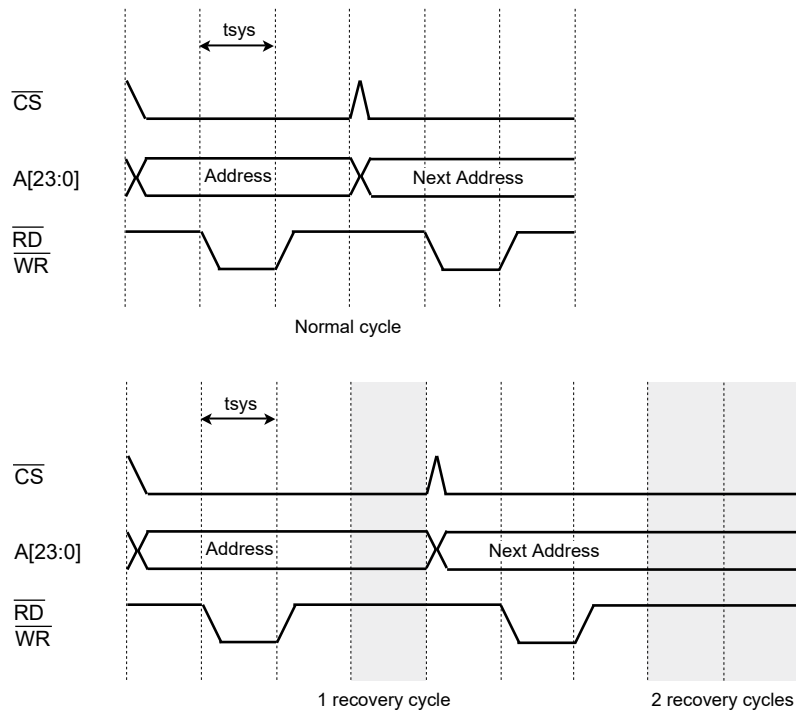
Figure 10-7 Timing of Recovery Time insertion
