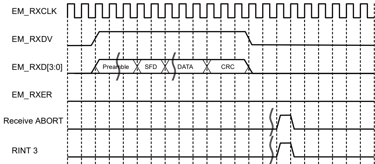
Figure 20-11 MII Frame Receive Timing (when a receive error and a short-frame error occur)
