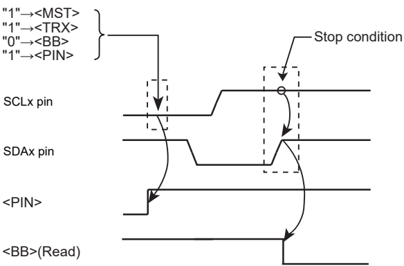
Figure 14-13 Generating the Stop Condition
