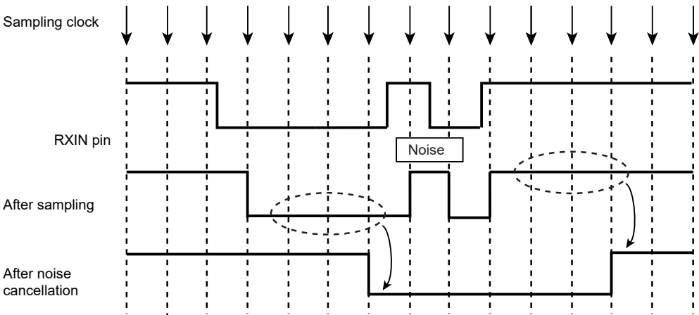
Figure 21-3 Noise Cancel (In the case of RMCRCR4="0011" (3 Cycles))
