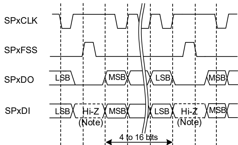
Figure 15-8 SPI frame format (continuous transfer, \langle SPO \rangle = 1 & \langle SPH \rangle = 0 )
