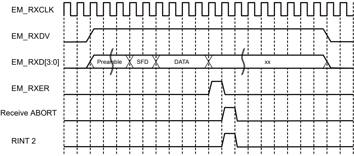
Figure 20-10 MII FFrame Receive Timing (when receive error occurred and EM_RXER is asserted)
