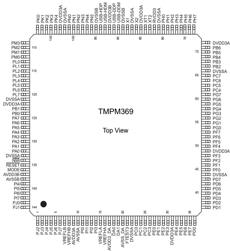
Figure 1-2 Pin Layout
