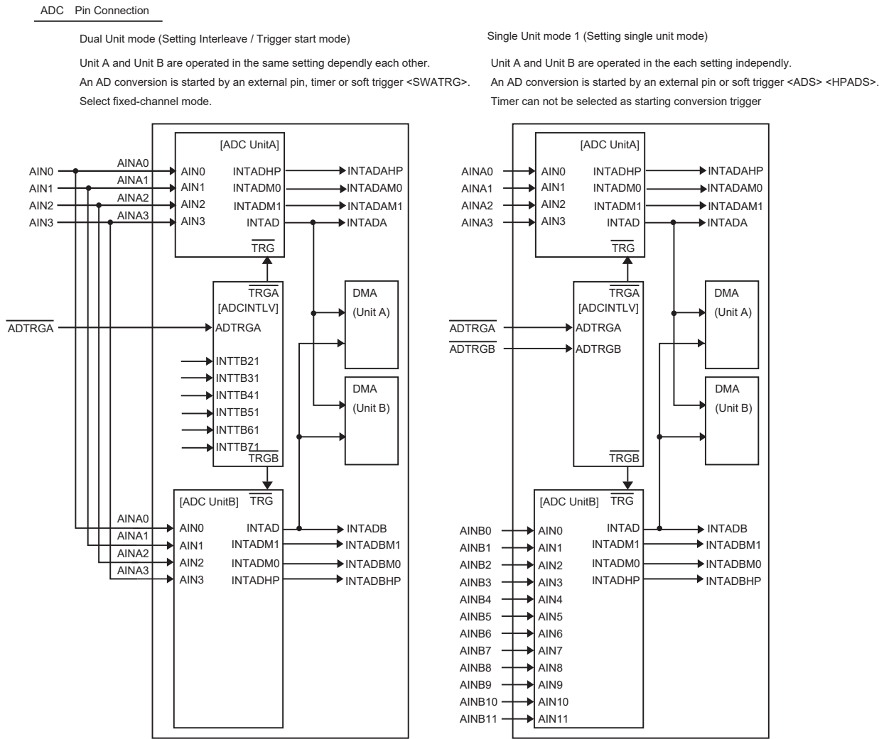
Figure 22-1 AD Converter Block Diagram
