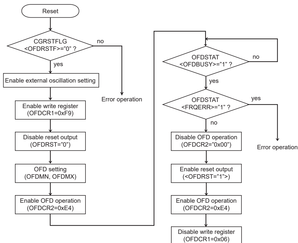
Figure 29-3 Example of operational procedure
