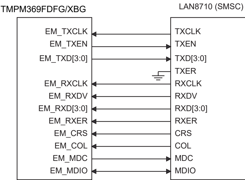
Figure 20-17 Example of connection ti LAN8710
