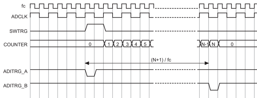
Figure 22-7 Interleave operation using a software trigger (ADCLK= f_c/2 )
