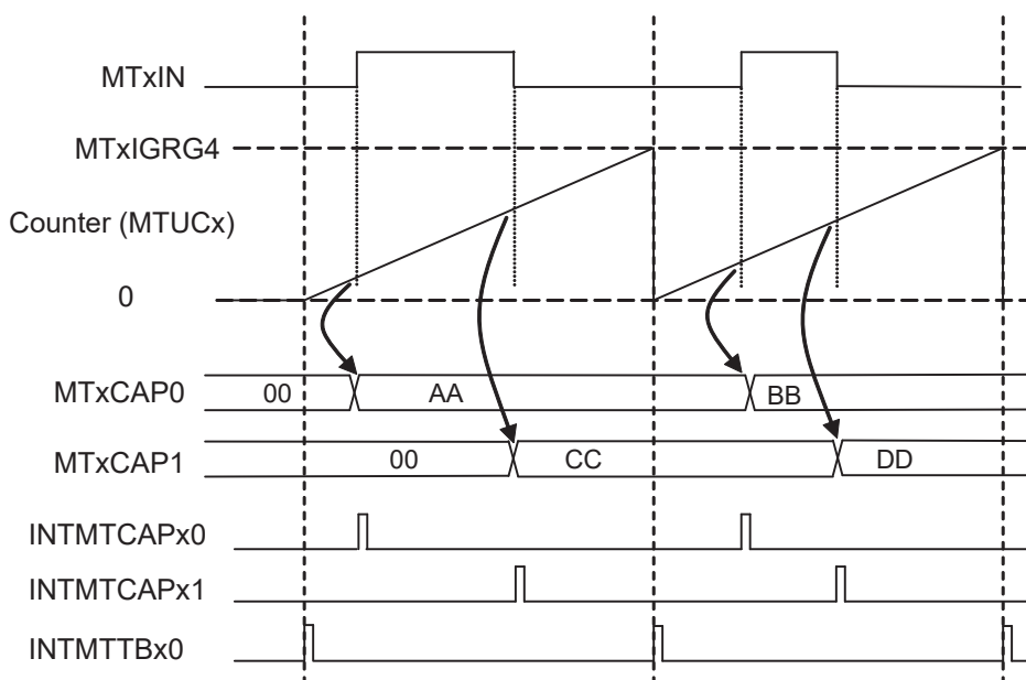
Figure 24-10 Capture operation
