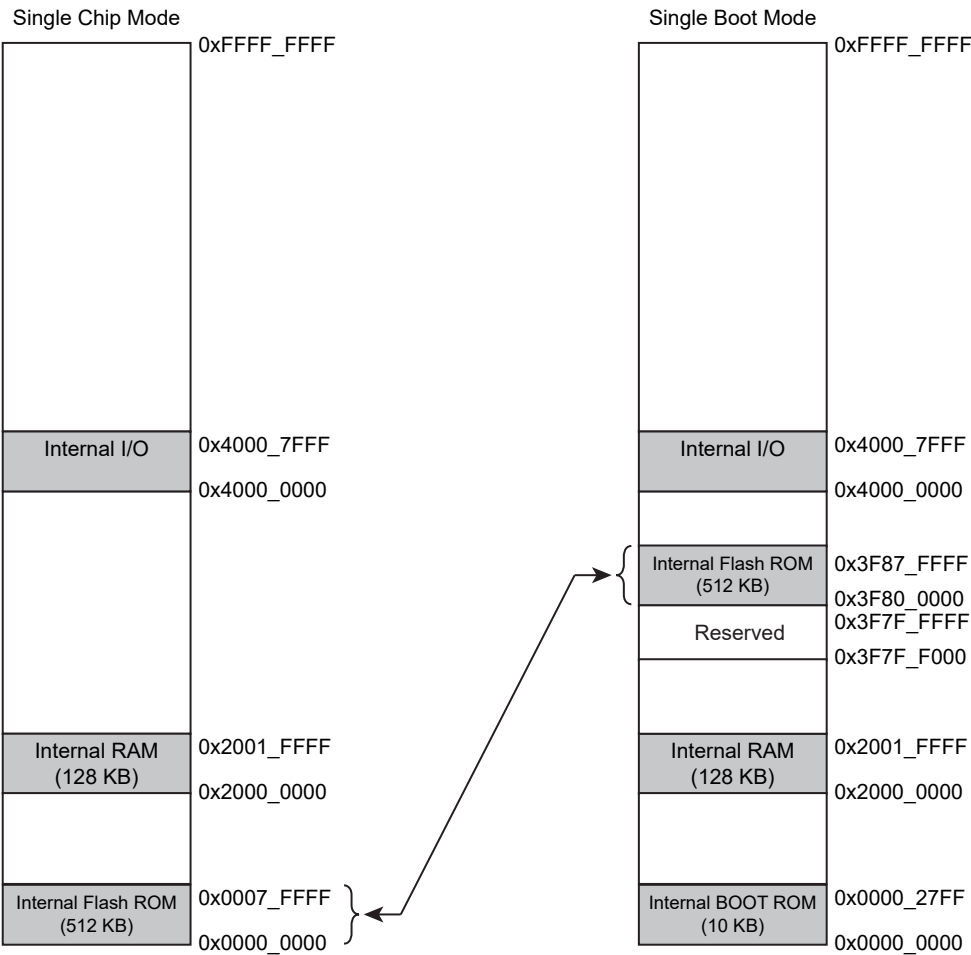
Figure 31-3 Memory Maps for TMPM369FDFG/XBG
