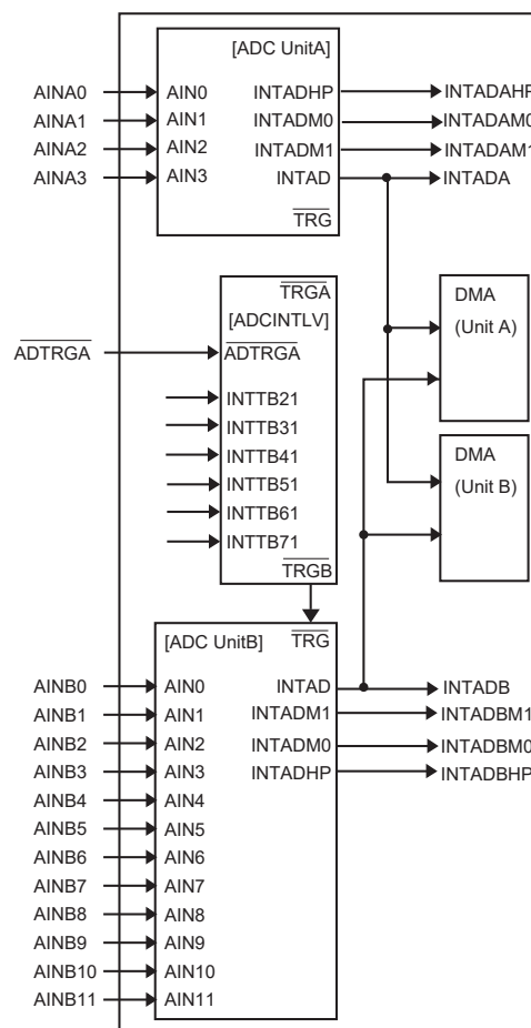
Figure 22-2 AD Converter Block Diagram
