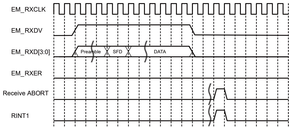
Figure 20-9 MII Frame Receive Timing (when a CRC error occurred and EM_RXDV is negated)
