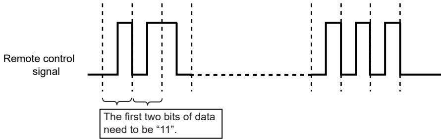
Figure 21-11 The waveform pattern in phase method
