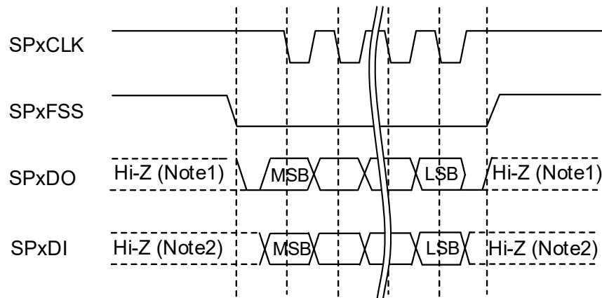
Figure 15-7 SPI frame format (single transfer, \langle SPO \rangle = 1 & \langle SPH \rangle = 0 )
