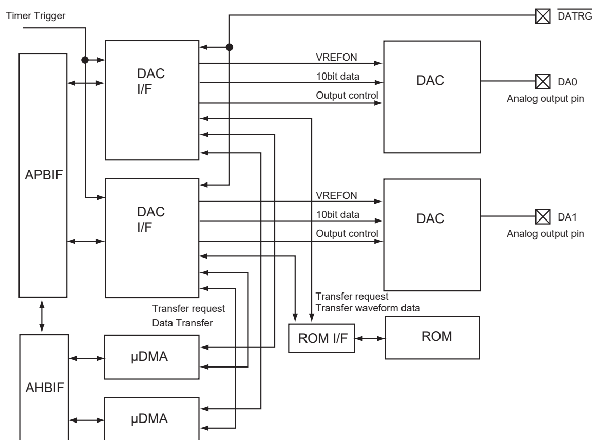
Figure 23-1 Block diagram of DAC
