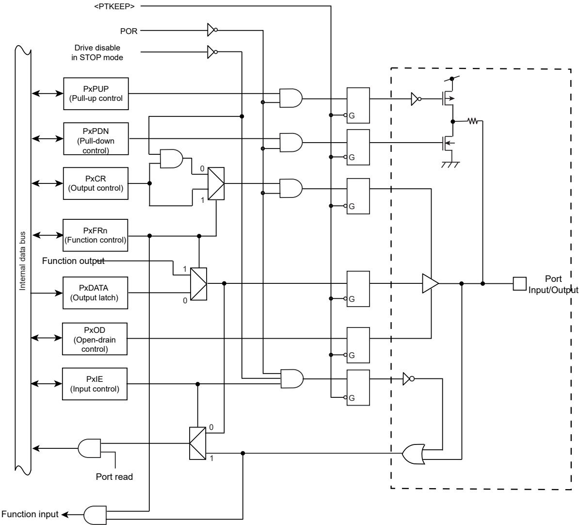
Figure 9-9 Port Type FT9
