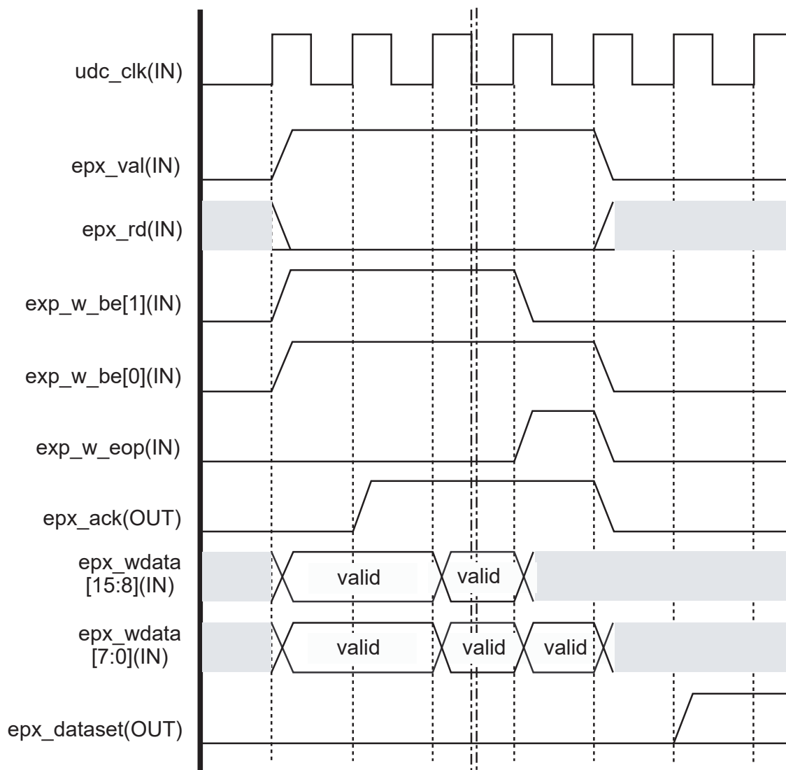
Figure 17-32 MPS (odd number) write access with max_pkt = even number (EP direct access)
