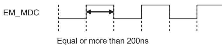
Figure 20-14 EM_MDC signal
