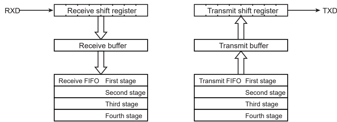
Figure 12-3 The Configuration of Buffer and FIFO
