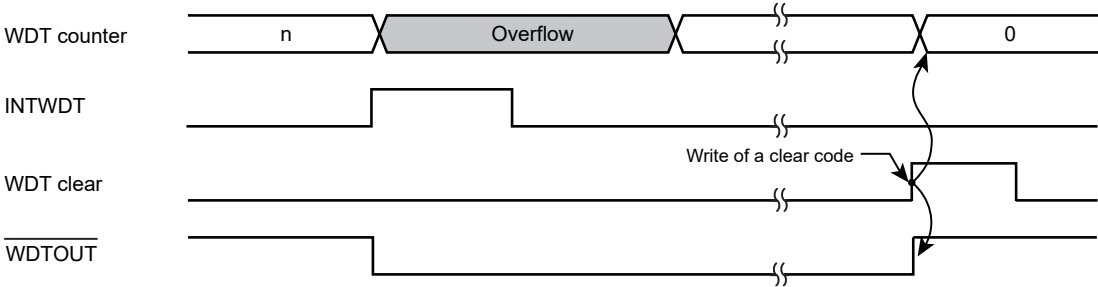
Figure 30-2 INTWDT interrupt generation
