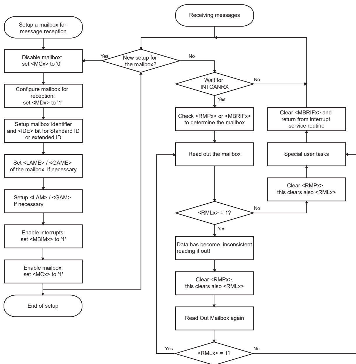
Figure 19-9 Flowchart of Message Reception
