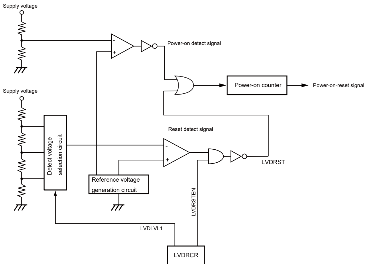
Figure 27-1 Power-on-reset circuit
