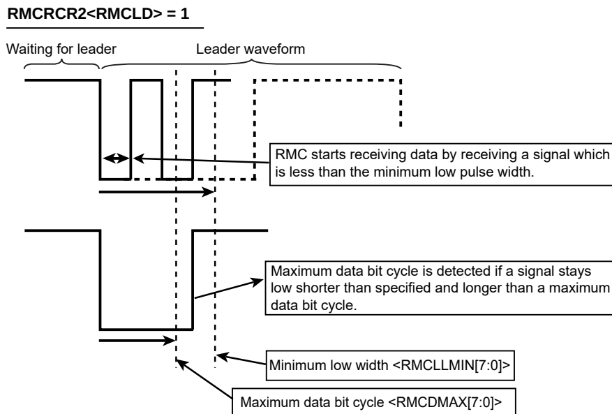
Figure 21-8 Receiving Remote Control RCR2<RMCLD>="1")
