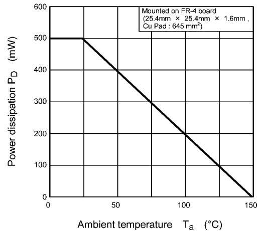
Fig. 7.12 P_D - T_a
