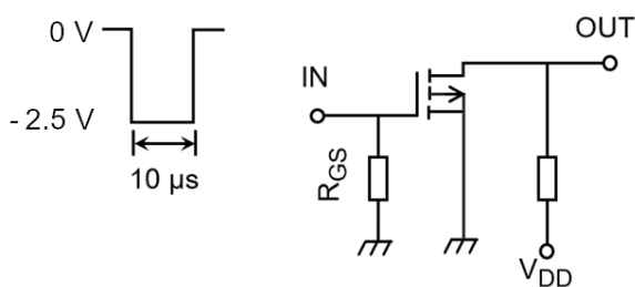
Fig. 5.3.1 Test Circuit of Switching Time
