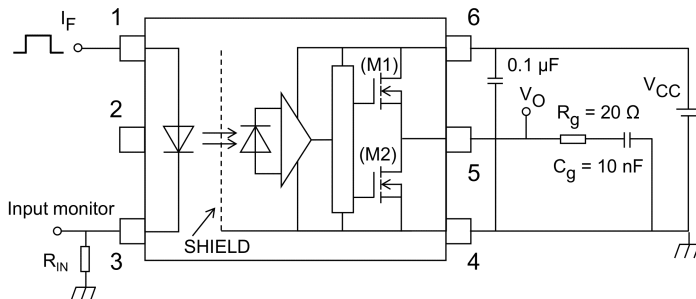
Fig. 13.1.8 Switching Time Test Circuit and Waveform
