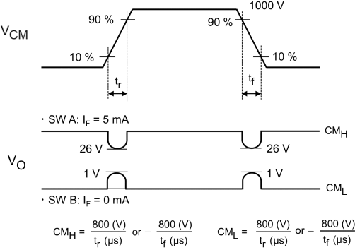
Fig. 13.1.9 Common-Mode Transient Immunity Test Circuit and Waveform
