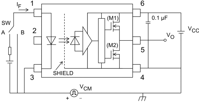
Fig. 13.1.9 Common-Mode Transient Immunity Test Circuit and Waveform
