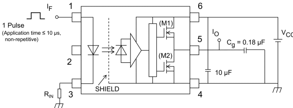
Fig. 13.1.7 I_{OLH} / I_{OHL} Test Circuit
