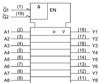
TC74ACT541FT
