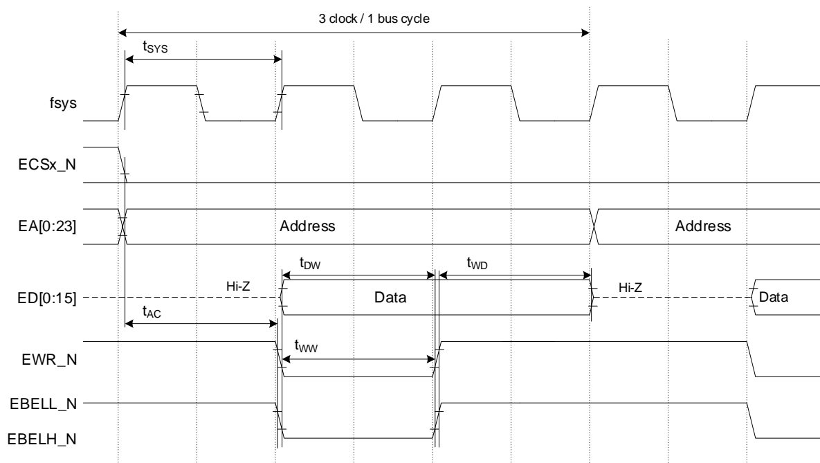
Figure 7.11 Write Cycle Timing (Minimum Cycle)
