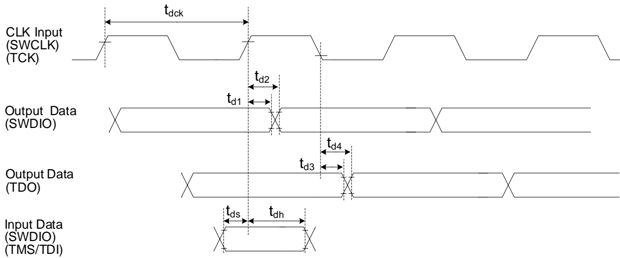
Figure 7.28 JTAG/SWD Waveform
