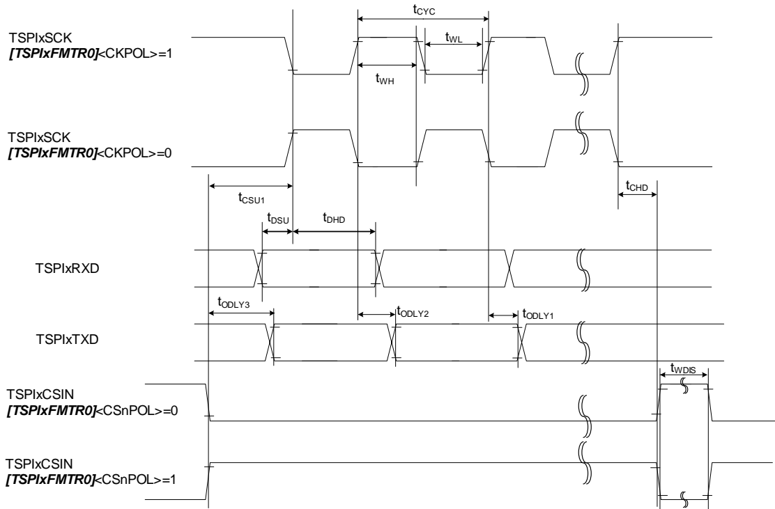
Figure 7.3 1st Clock Edge Sampling (Slave)
