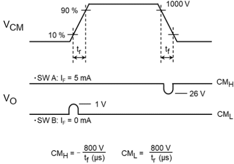
Fig. 13.1.8 Common-Mode Transient Immunity Test Circuit and Waveform
