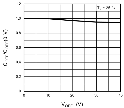
Fig. 12.10 C_{OFF}/C_{OFF}(0\text{ V}) - V_{OFF}
