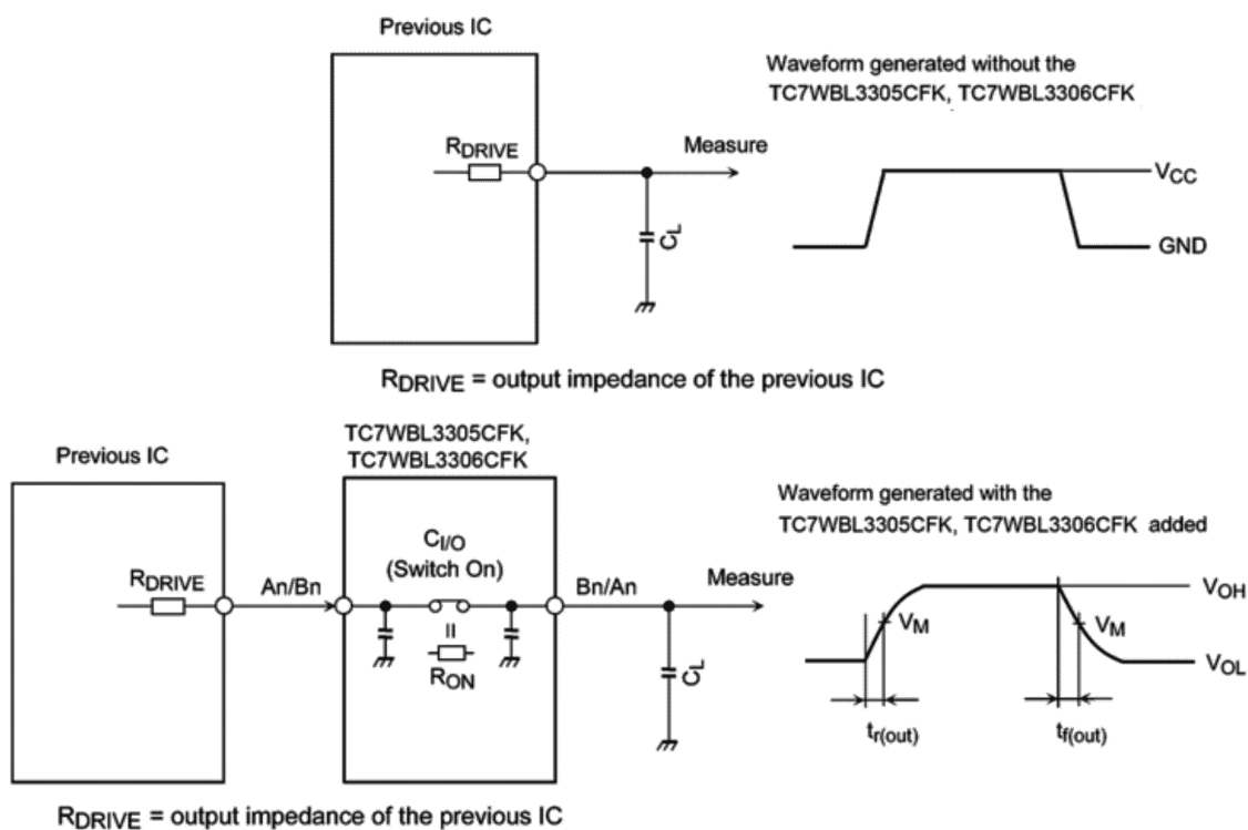
Fig. 12.1 Calculation Circuit
