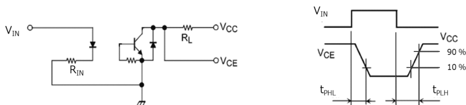
Fig. 10.1 Propagation delay Time Test Circuit and Waveform
