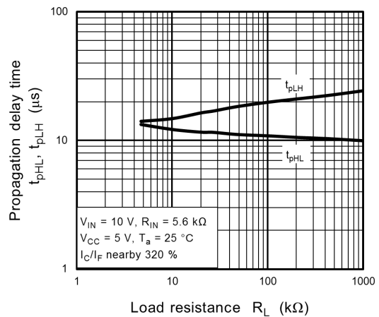
Fig. 11.16 Propagation Delay - R_L
