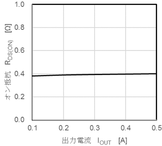
R_{DS(ON)} - I_{OUT}
