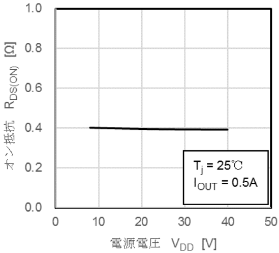
R_{DS(ON)} - V_{DD}
