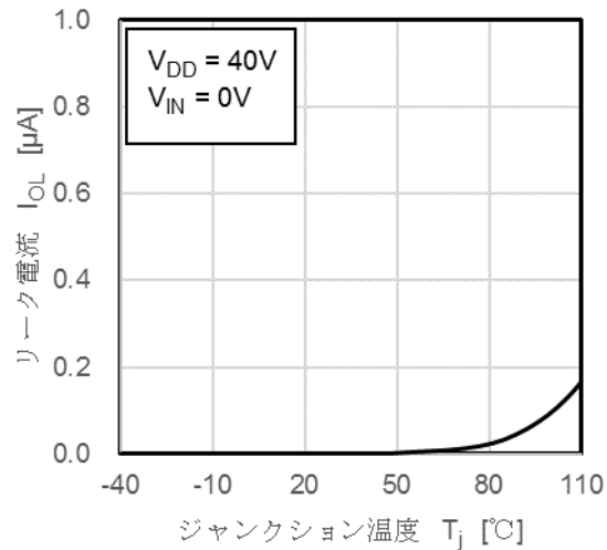
I_{OL} - T_j
