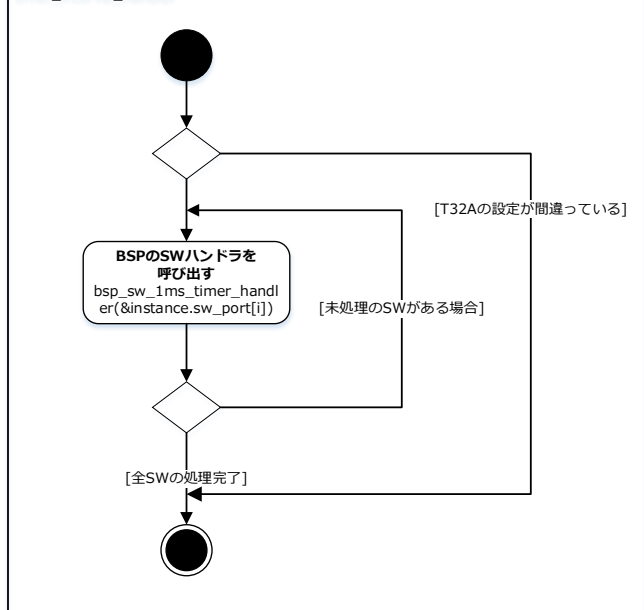
timer_interval_handler
