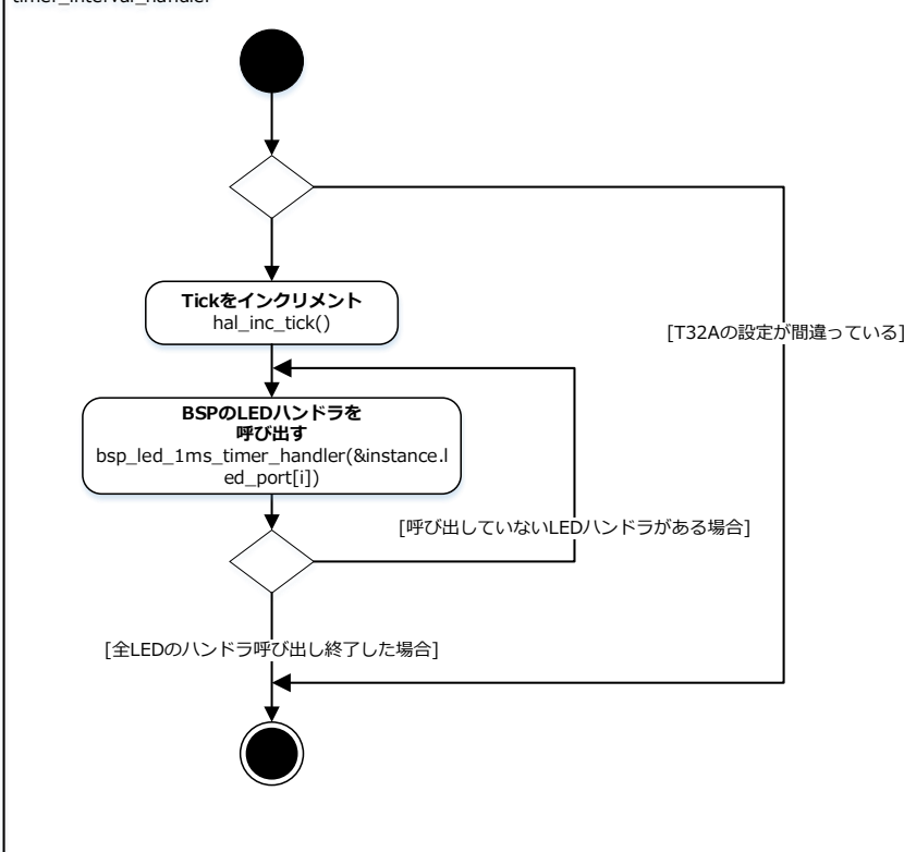
timer_interval_handler
