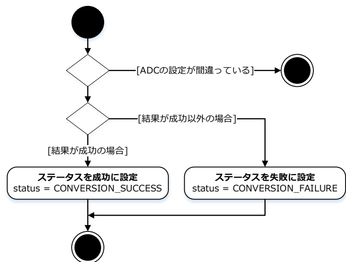
done_handler
