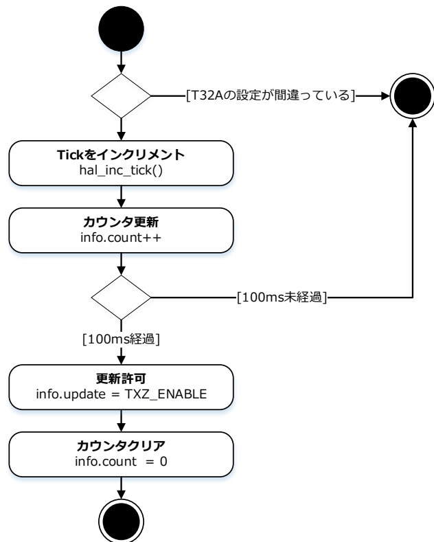
timer_interval_handler
