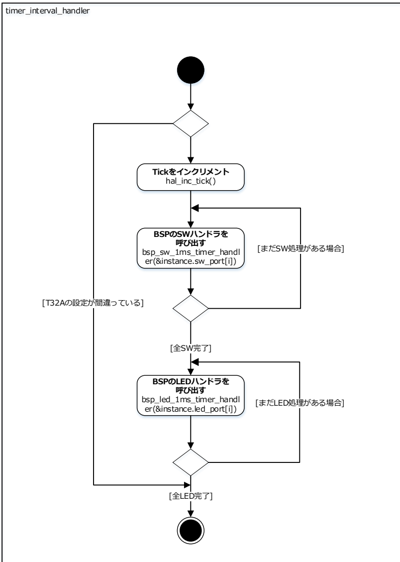
timer_interval_handler
