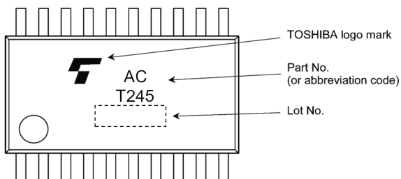
TC74ACT245FT
