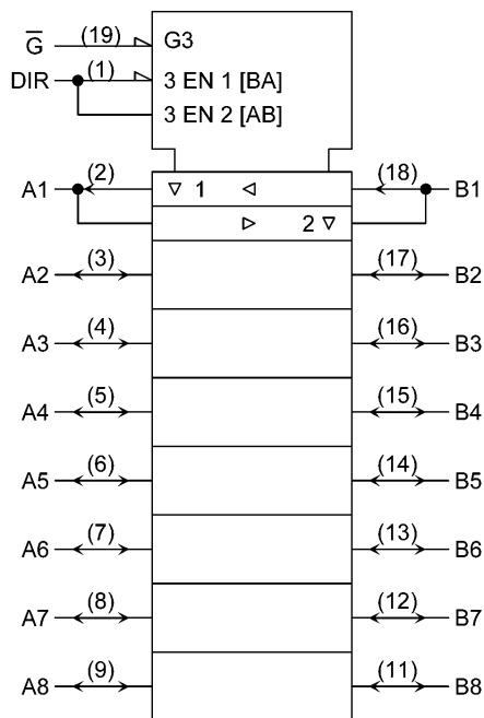
TC74ACT245FT
