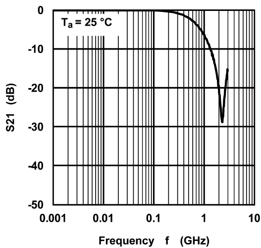
図 10.1 S_{21} - f
