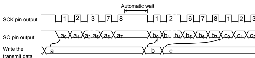
Fig. 12-24 Automatic Wait
