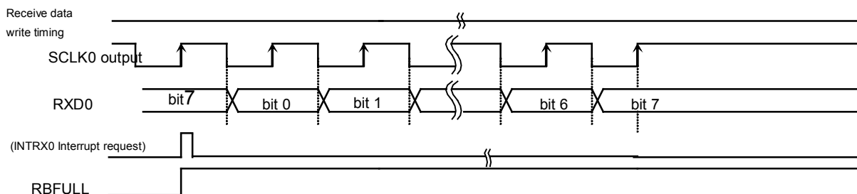
Fig. 11-12 Receive Operation in the I/O Interface Mode (SCLK0 Output Mode)
