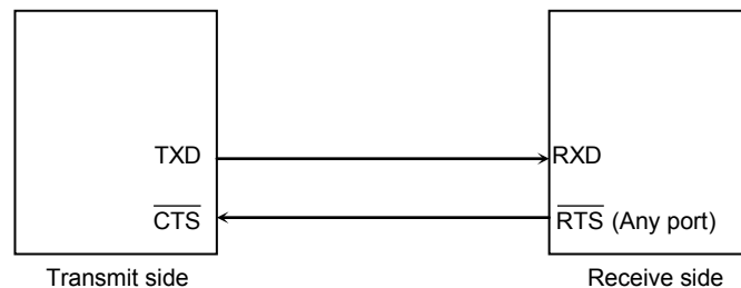
Fig. 11-6 Handshake Function
