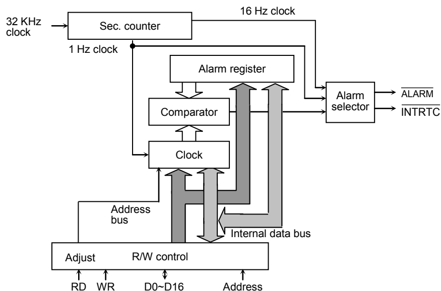
Fig. 17-1 Block Diagram
