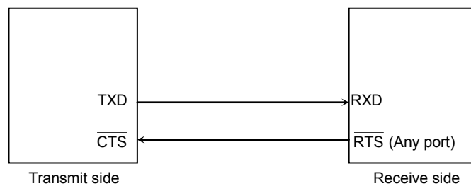
Fig. 11-6 Handshake Function
