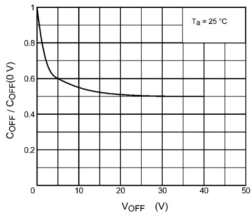
Fig. 12.1.10 C_{OFF}/C_{OFF}(0\text{V}) - V_{OFF}
