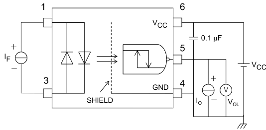
Fig. 12.1.1 V_{OL} Test Circuit
