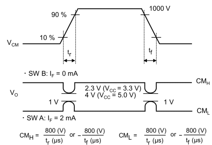
Fig. 12.1.6 Common-Mode Transient Immunity Test Circuit and Waveform
