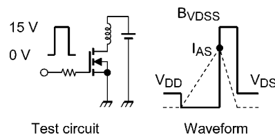
Fig. 8.15 Test Circuit/Waveform
