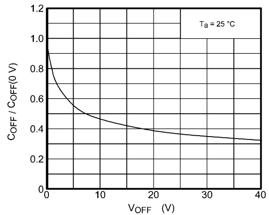
Fig. 12.1.10 C_{OFF}/C_{OFF}(0\text{ V}) - V_{OFF}
