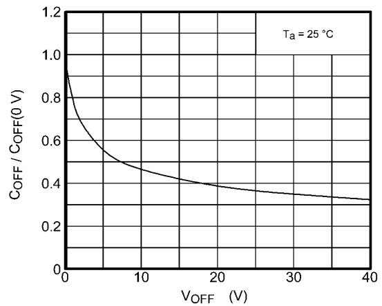
図 12.1.10 C_{OFF}/C_{OFF}(0 V) - V_{OFF}
