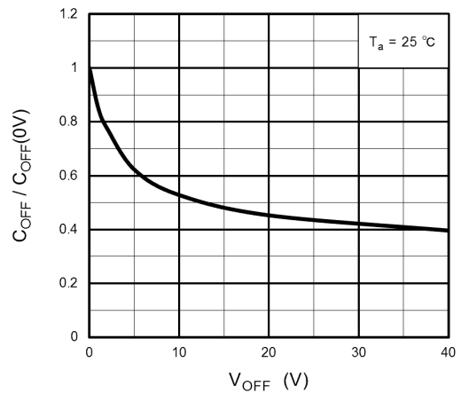
図 12.1.10 C_{OFF}/C_{OFF}(0\text{V}) - V_{OFF}
