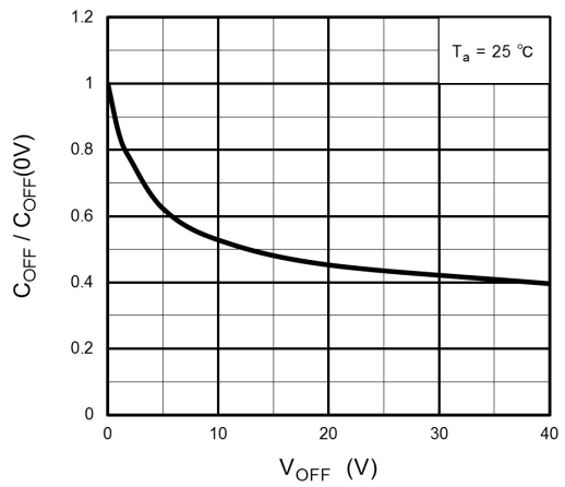
図 12.1.10 C_{OFF}/C_{OFF}(0V) - V_{OFF}
