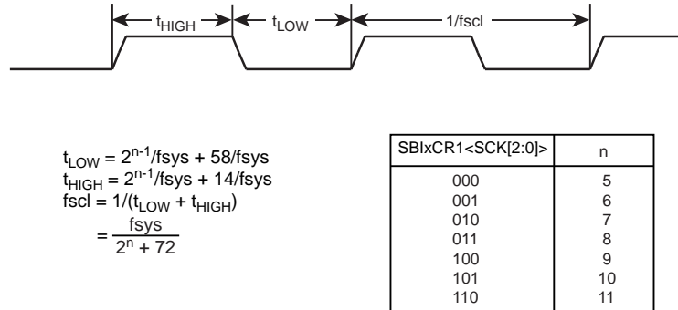
Figure 15-3 Clock source
