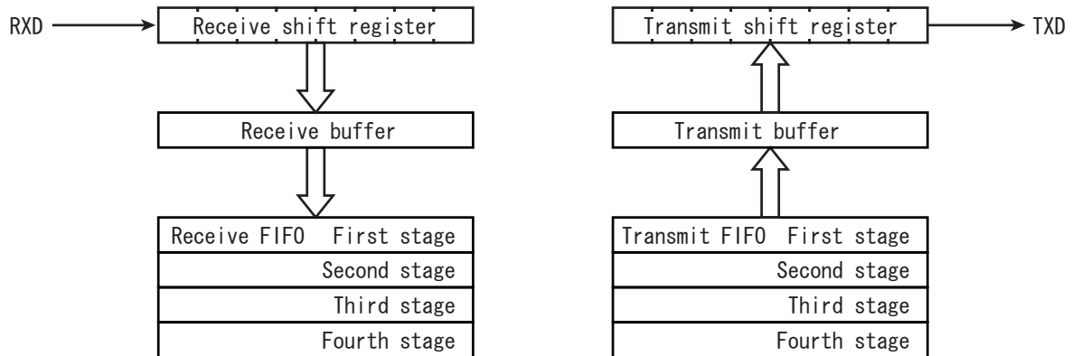
Figure 14-3 The Configuration of Buffer and FIFO
