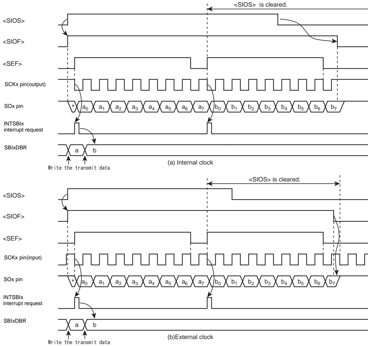
Figure 15-22 Transmit Mode
