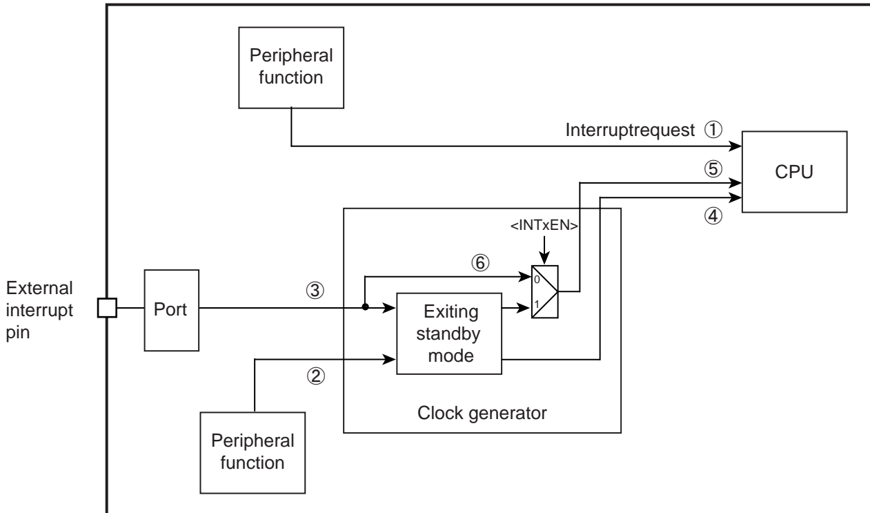
Figure 9-1 Interrupt Route
