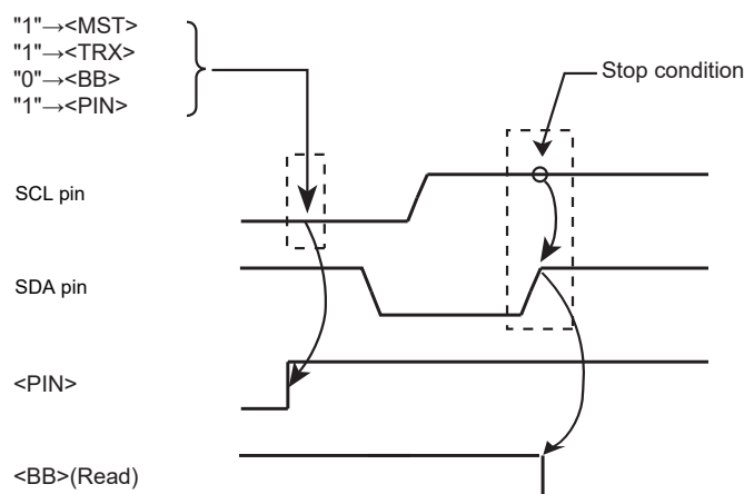
Figure 15-13 Generating the Stop Condition
