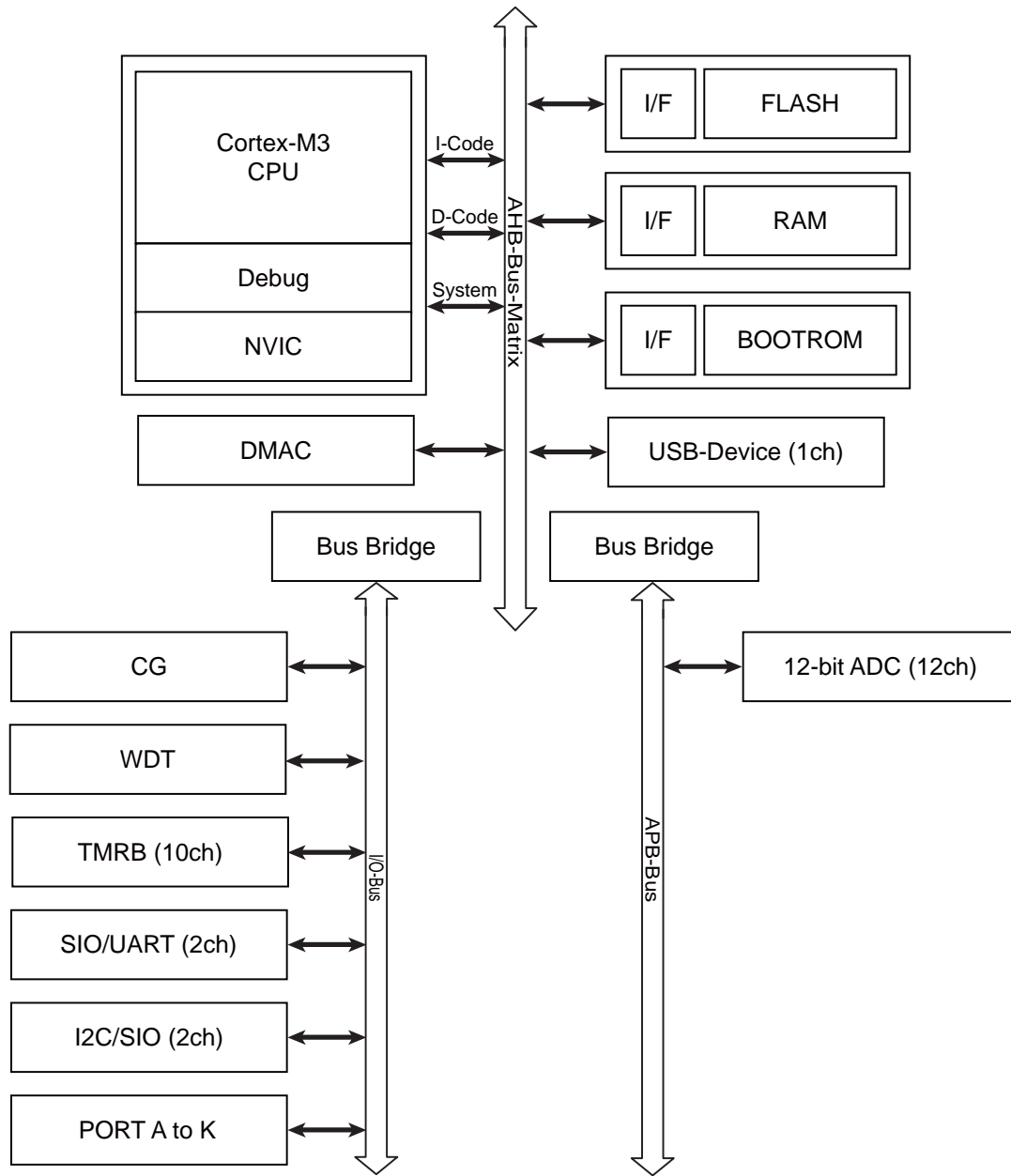
Figure 1-1 TMPM365FYXBGBlock Diagram
