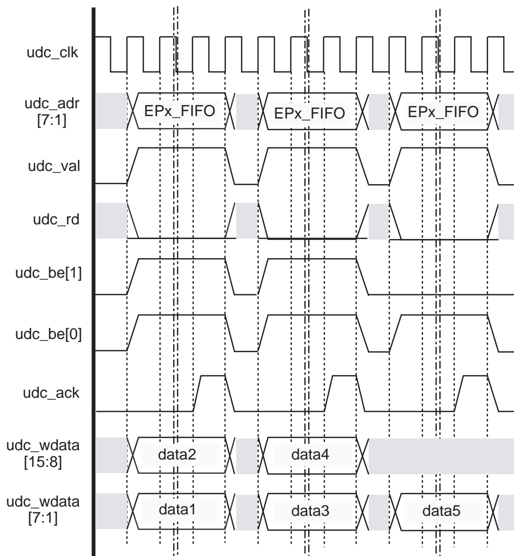
Figure 13-31 MPS write access with max_pkt = odd number (common bus access)
