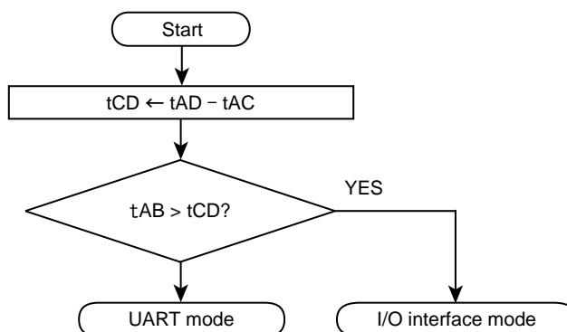
Figure 17-8 Serial operation mode determination flowchart
