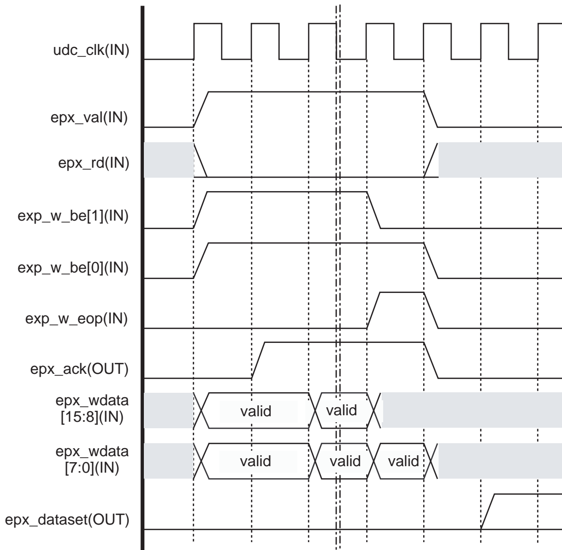
Figure 13-32 MPS (odd number) write access with max_pkt = even number (EP direct access)
