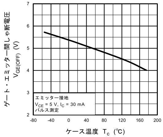
図 8.8 V_{GE(OFF)} - T_c
