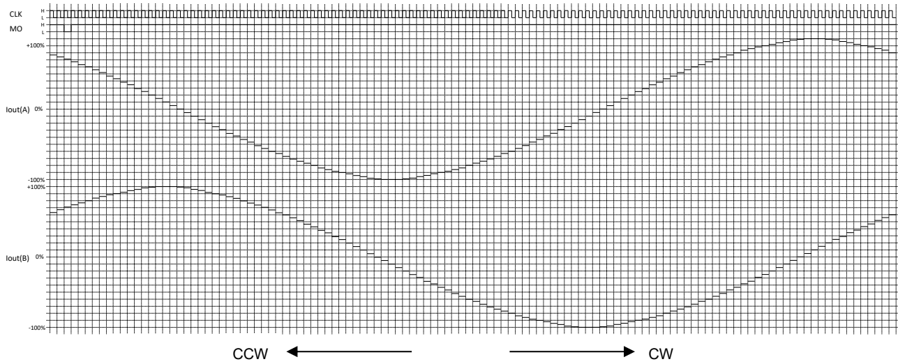
Figure 6.7 1/32 step resolution
