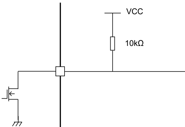
Figure 6.8 LO terminal
