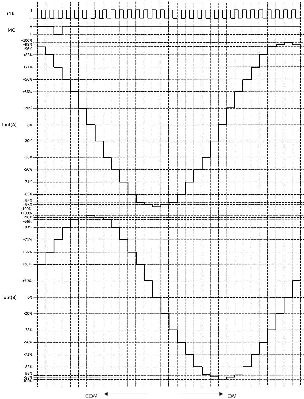
Figure 6.5 1/8 step resolution
