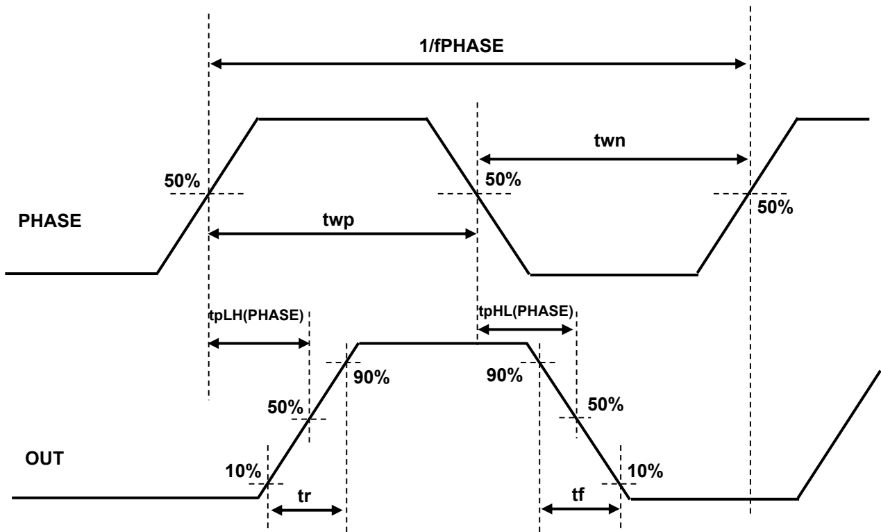
Figure 9.1 AC Electrical Specification Timing chart
