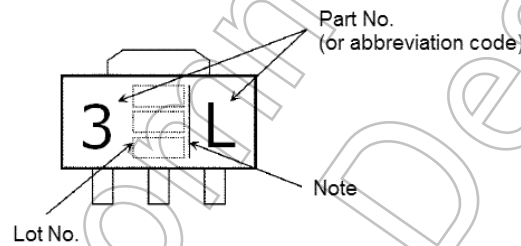
Fig. 6.1 Marking
